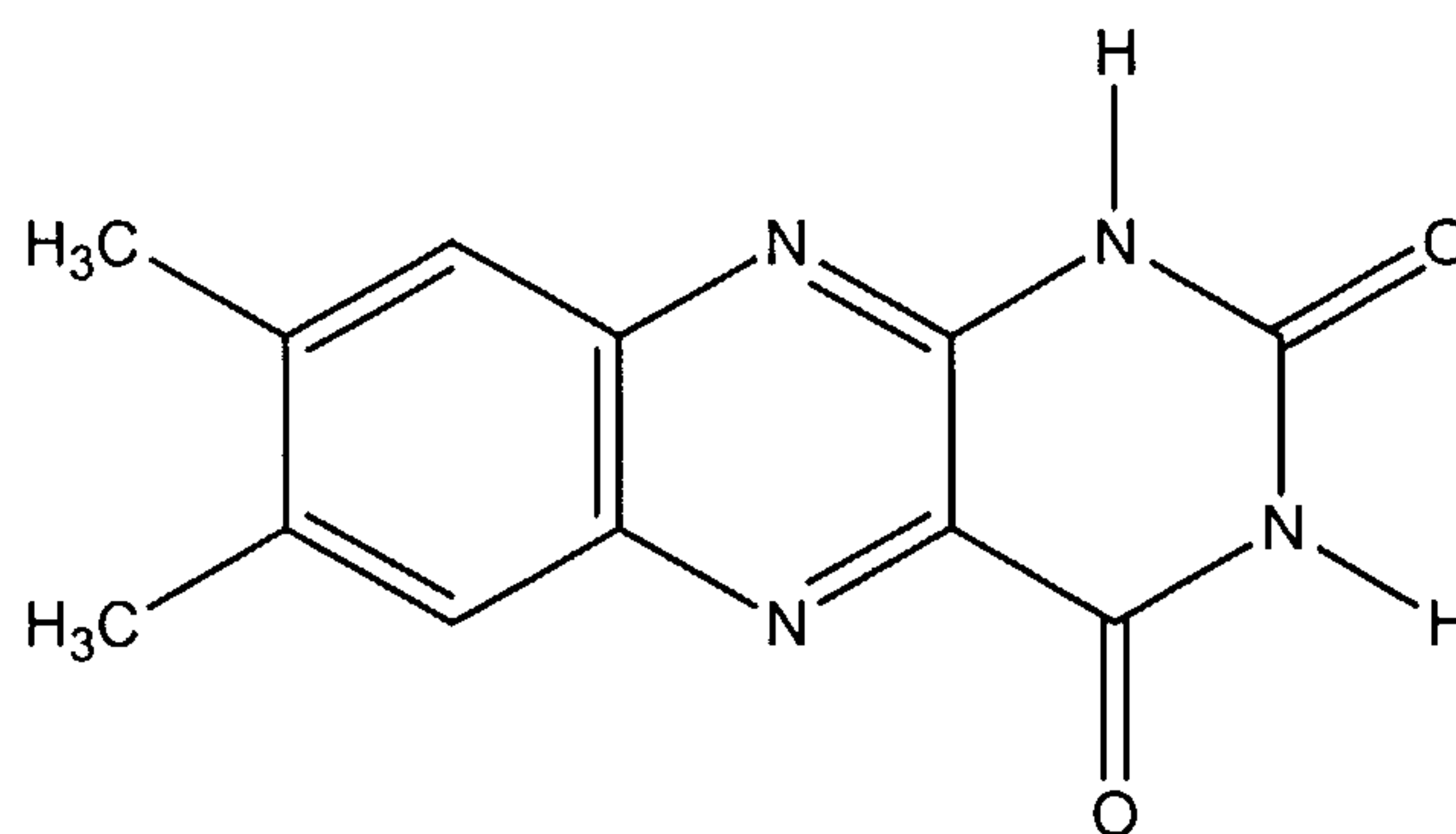
7,8-dimethylalloxazine
