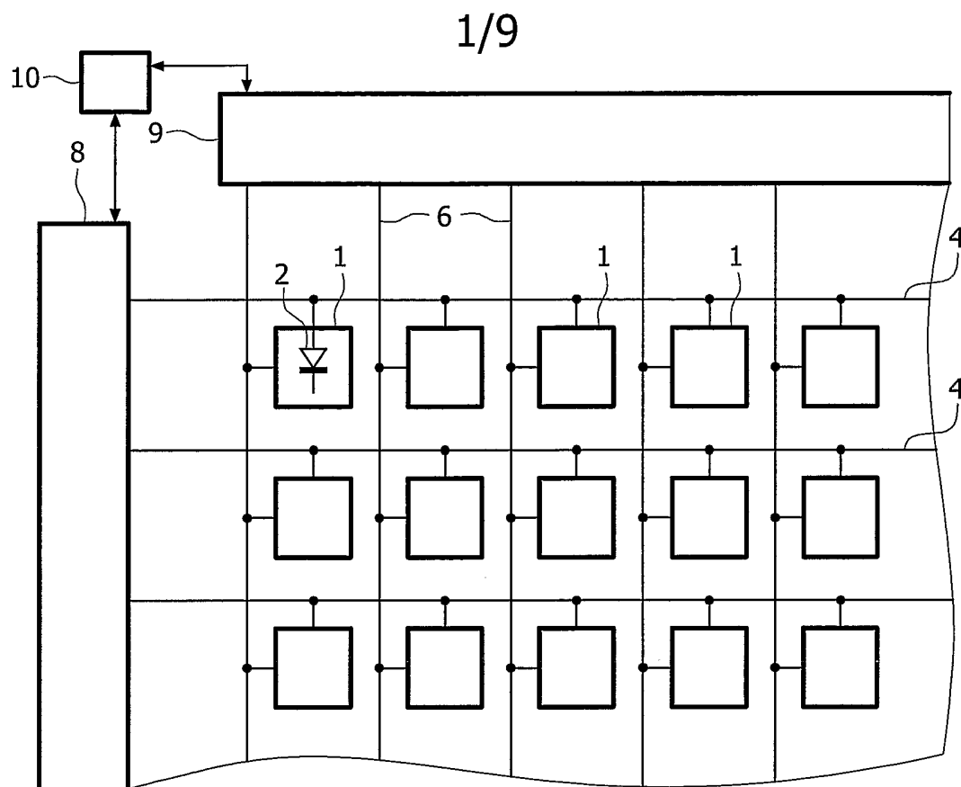
FIG. 1 PRIOR ART
