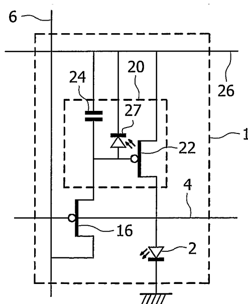
FIG. 2 PRIOR ART
