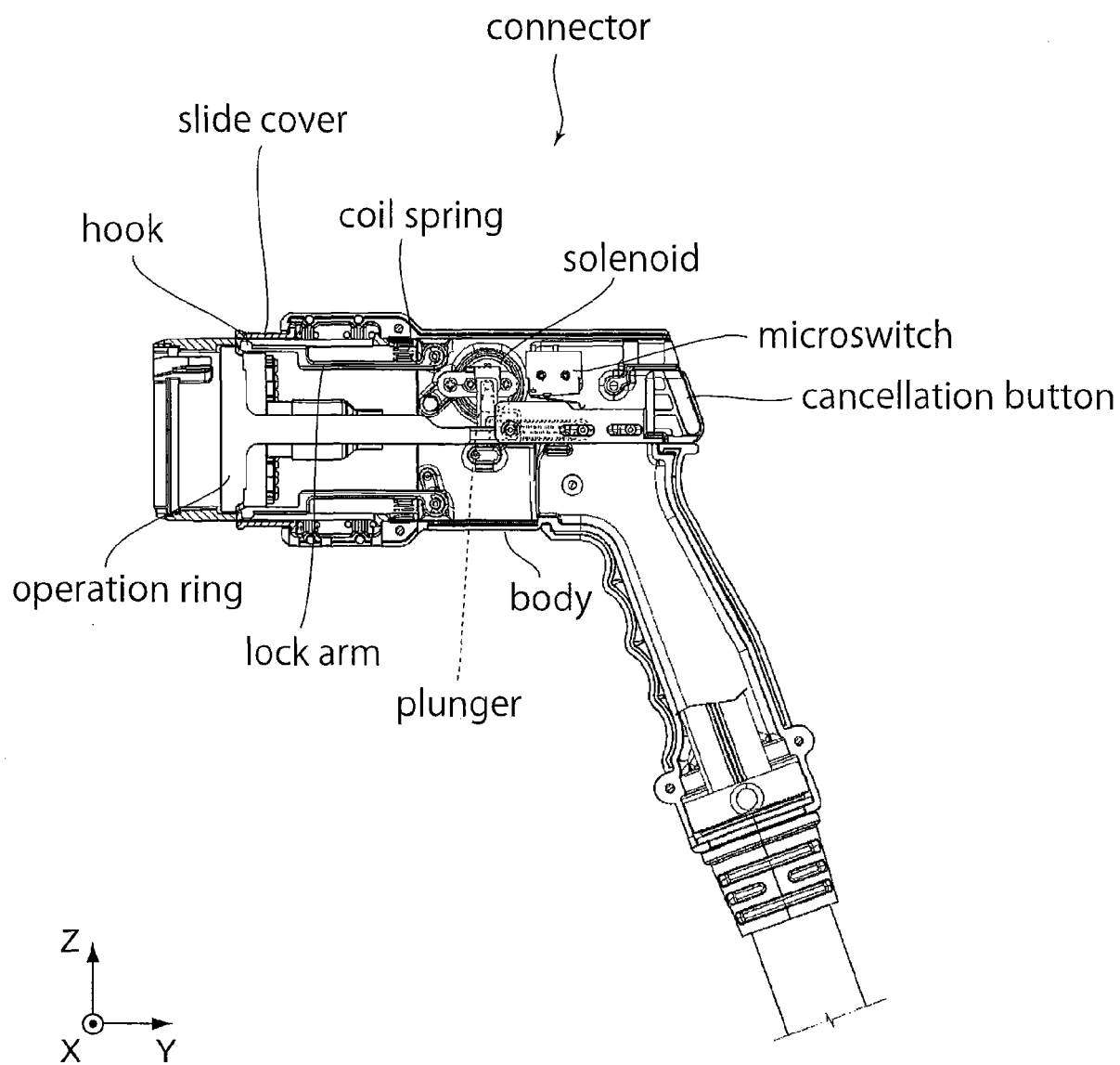
FIG. 21 PRIOR ART
