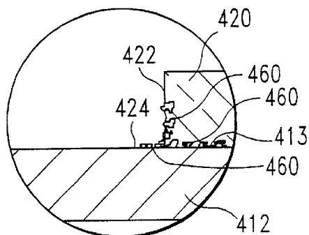
FIG. 4C (PRIOR ART)
