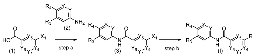
Reaction Scheme I:
