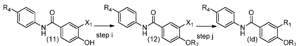
Reaction Scheme V:
