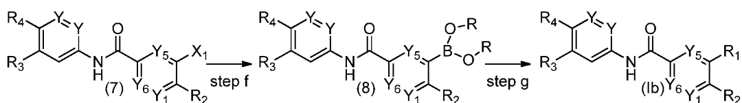
Reaction Scheme III:
