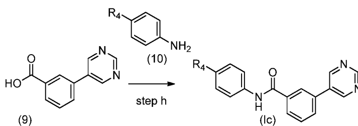
Reaction Scheme IV:
