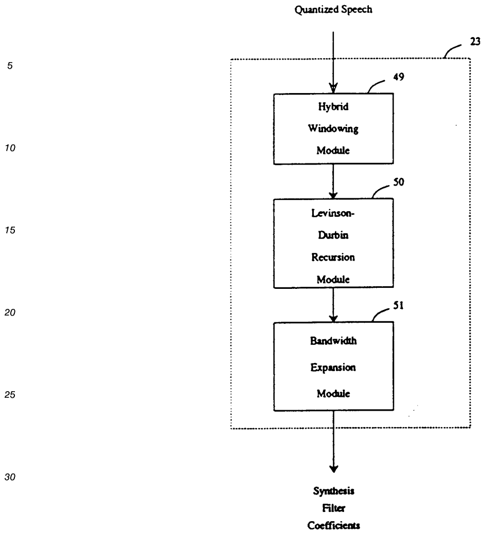
Figure 5/G.728 Backward Synthesis Filter Adapter
