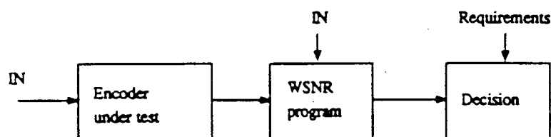
FIGURE I-3/G.728
