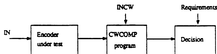
FIGURE I-1/G.728
