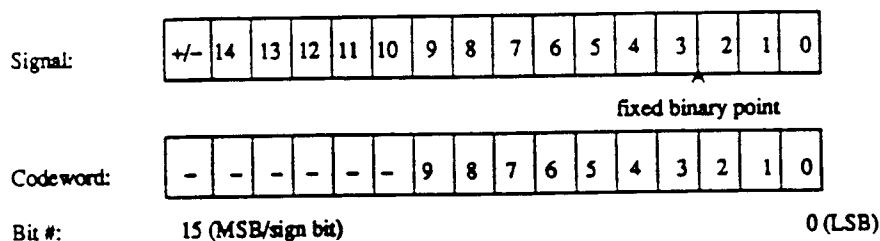
FIGURE I-5/G.728
