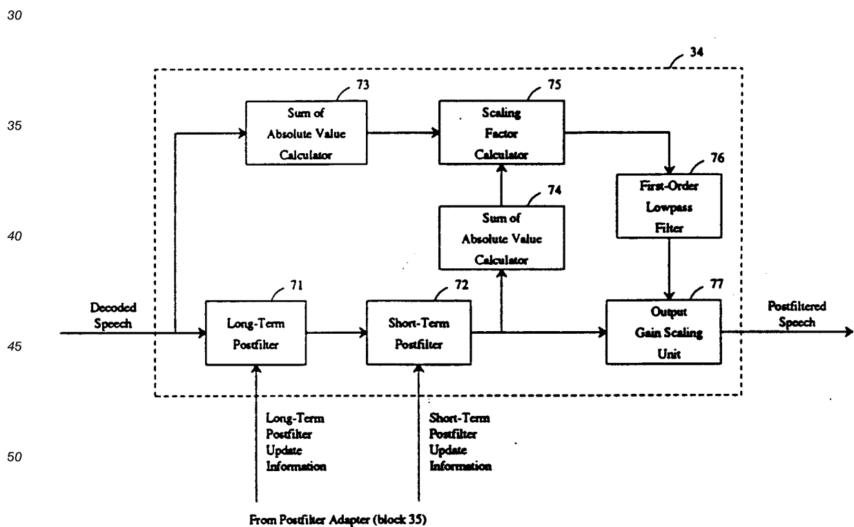
Figure 7/G.728 Postfilter Block Schematic
