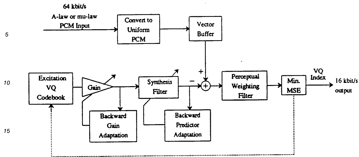
LD-CELP Encoder
