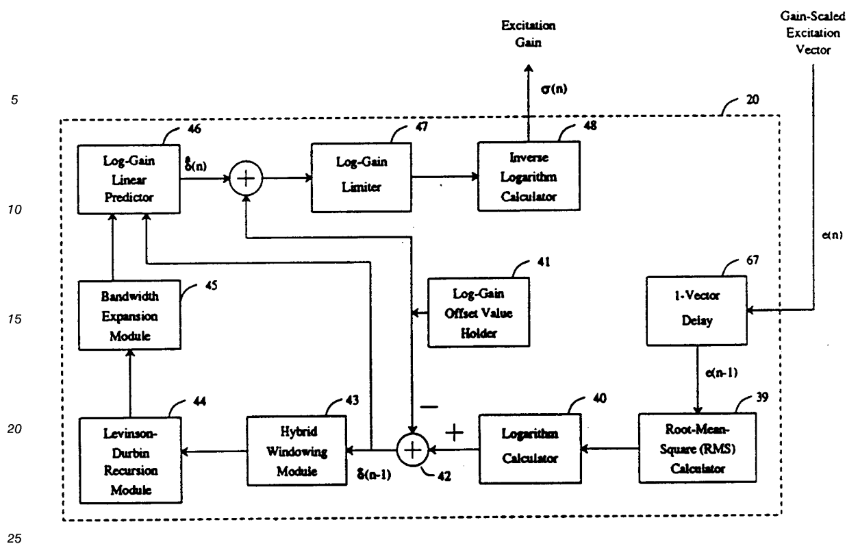
Figure 6/G.728 Backward Vector Gain Adapter
