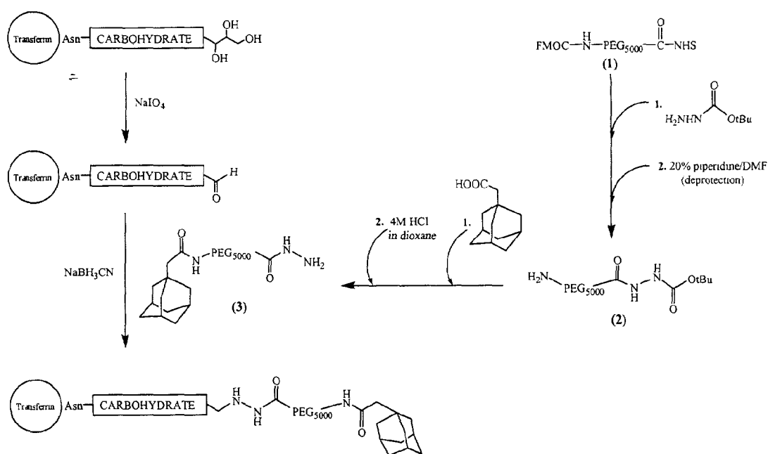
Figure 20 Synthesis of Adamantane-PEG-Transferrin (Ad-PEG-Tf)
