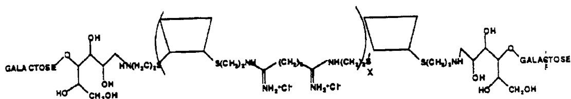
Fig. 2 Structure of Lactose-CDP6.
