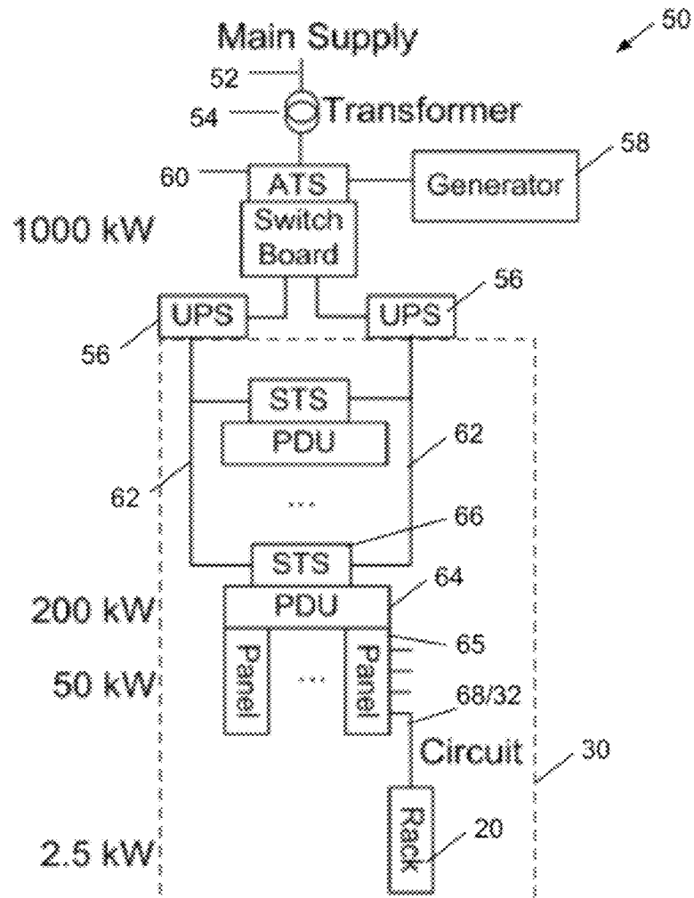
Figure 2 Simplified datacenter power distribution hierarchy.
