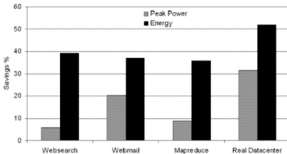
Figure 16: Power and energy savings achievable by reducing idle power consumption to 10% of peak
