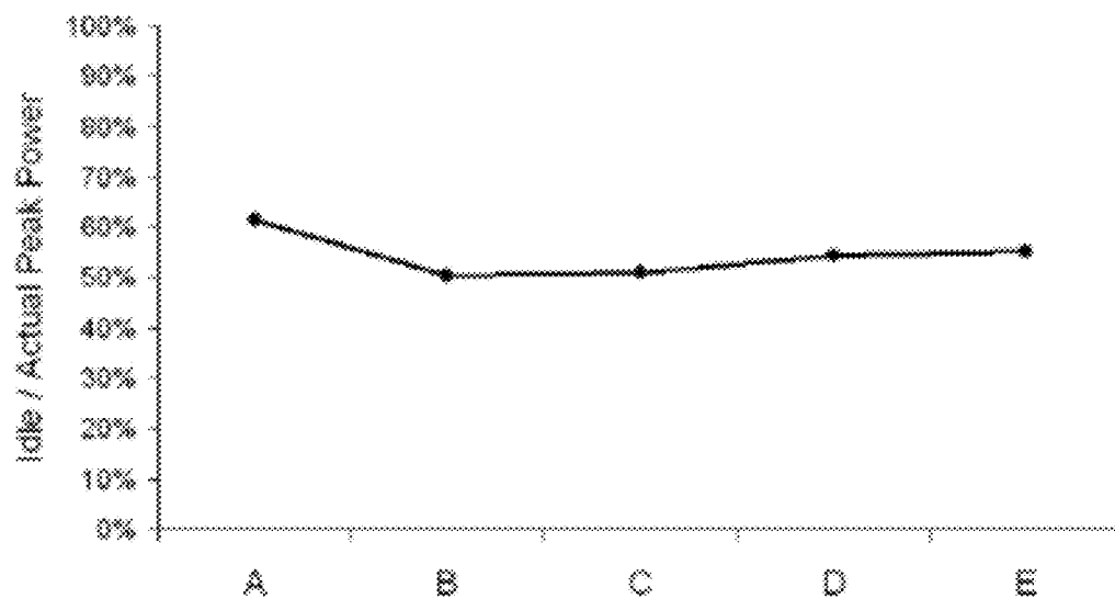
Figure 15: Idle power as fraction of peak power in 5 server configurations
