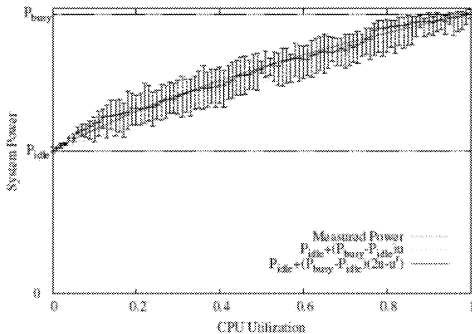
Figure 6: Model fitting at the machine level
