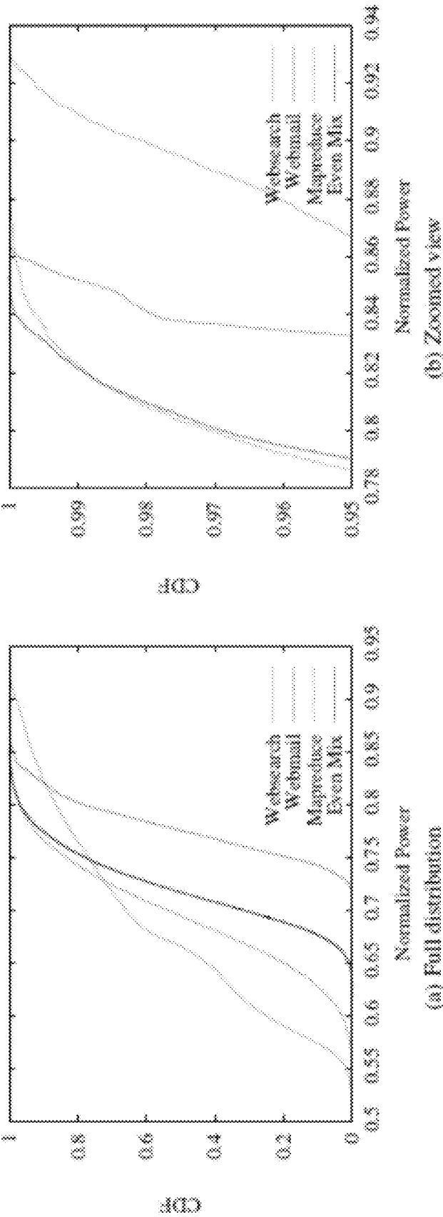
Figure 12: CDF of Websearch, Webmail, Mapreduce and the mixture of all at the cluster level
