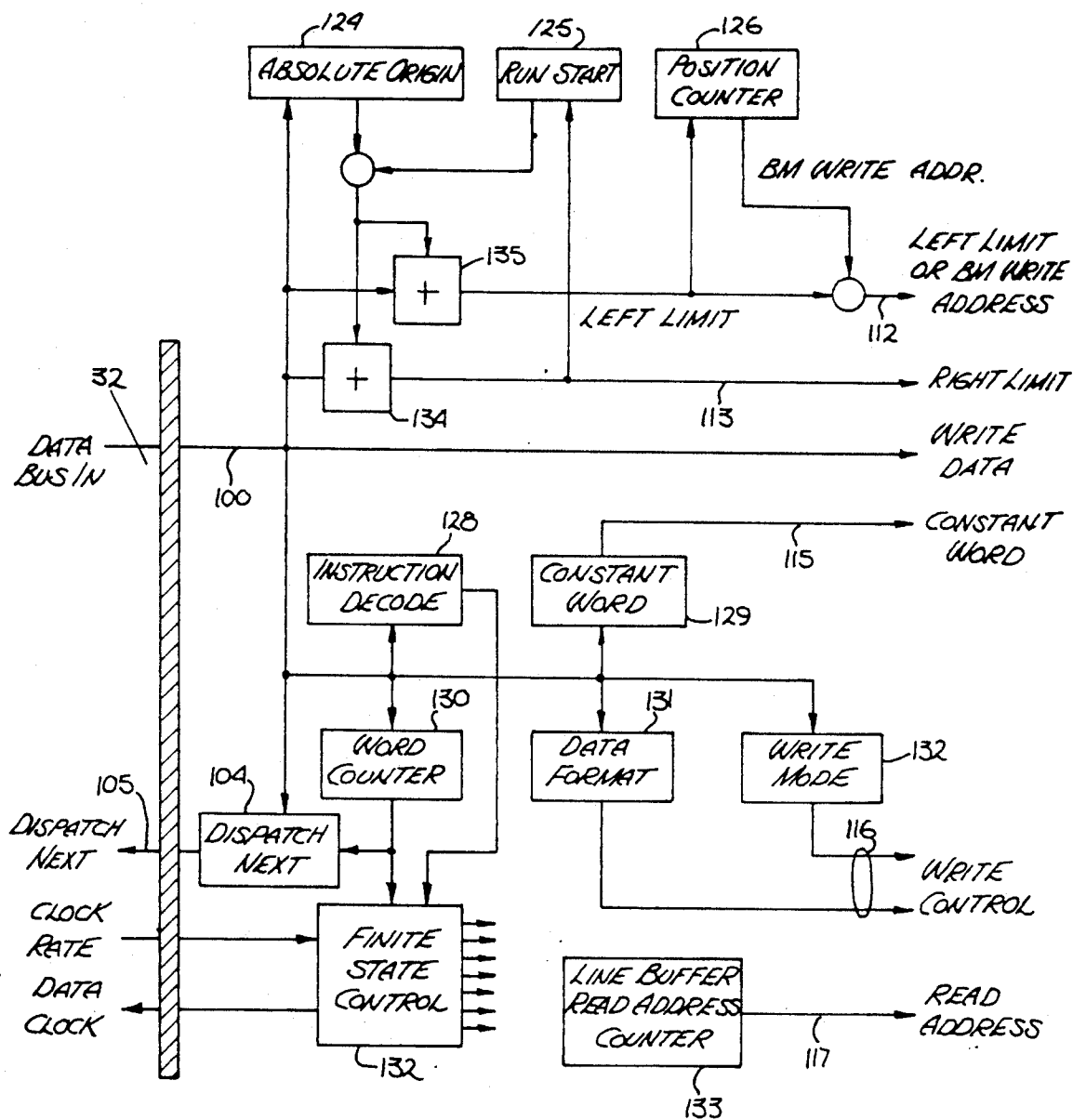
LINE BUFFER CONTROLLER
