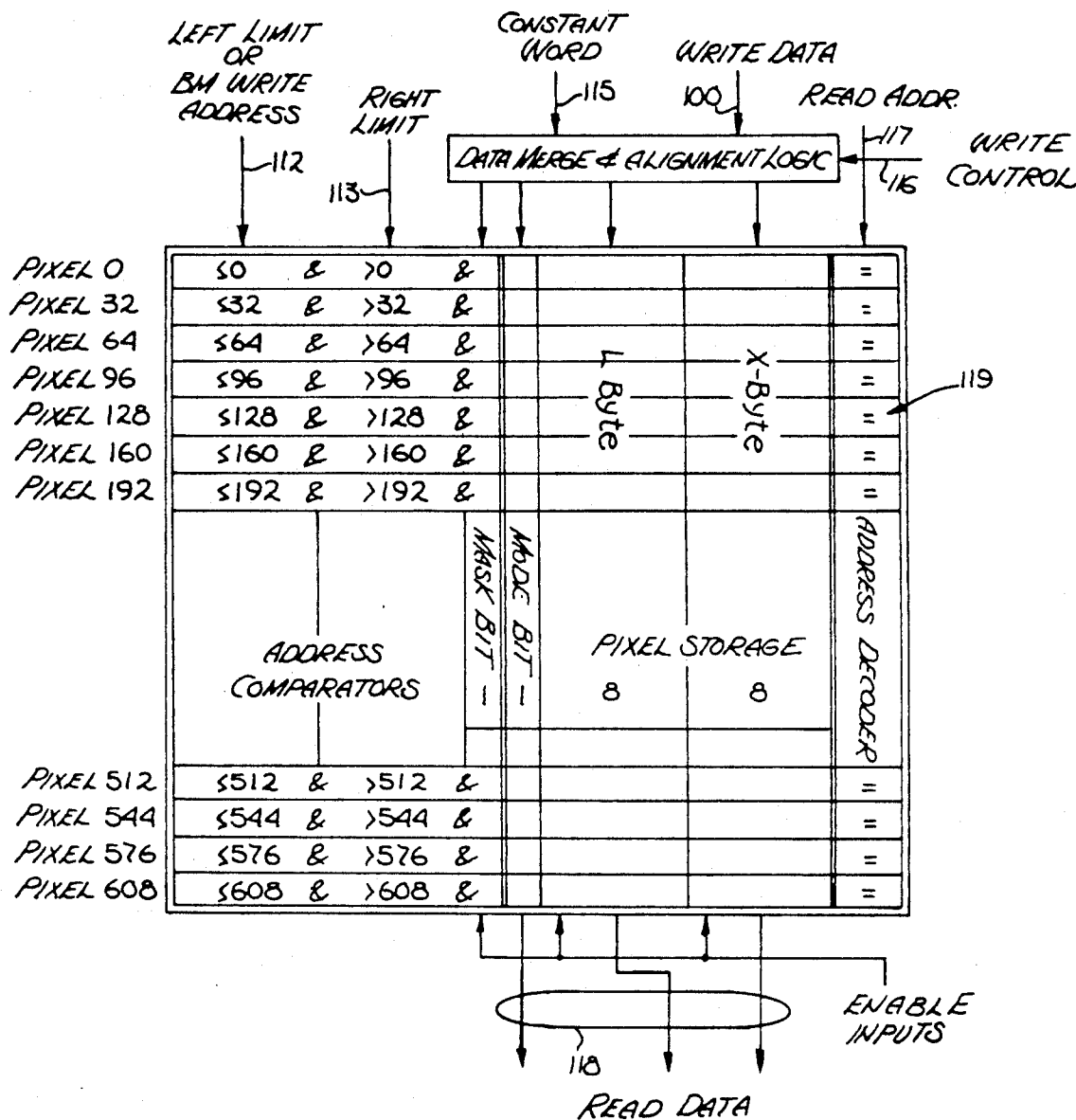
LINE BUFFER MEMORY CELL FOR MEMORY CELL GROUP ZERO
