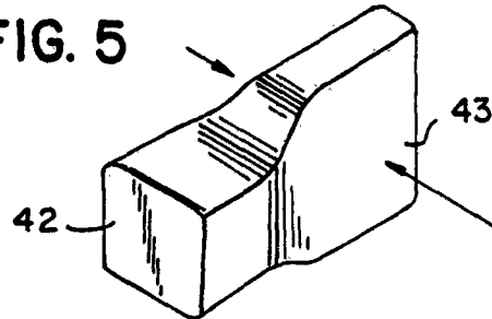
FORGING ROLL
