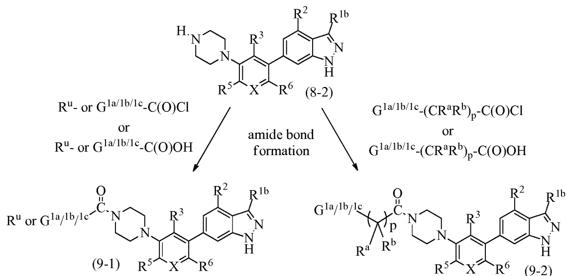
Scheme 9
