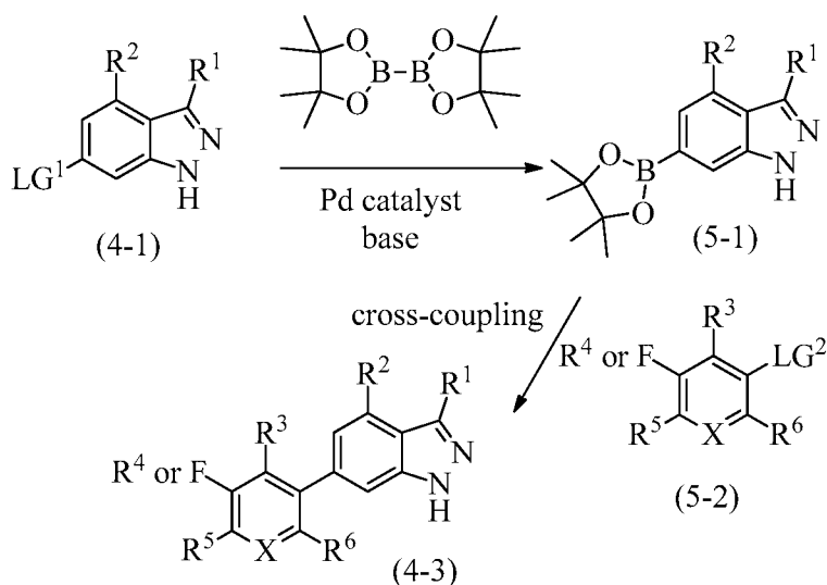
Scheme 5
