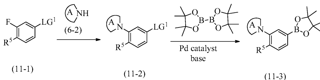
Scheme 11
