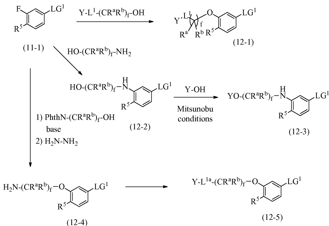
Scheme 12
