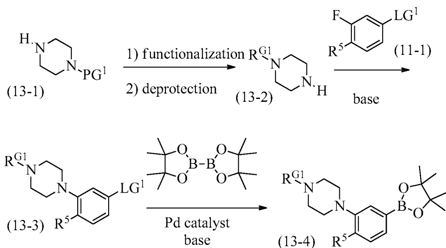
Scheme 13
