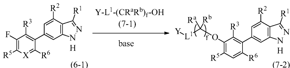
Scheme 7
