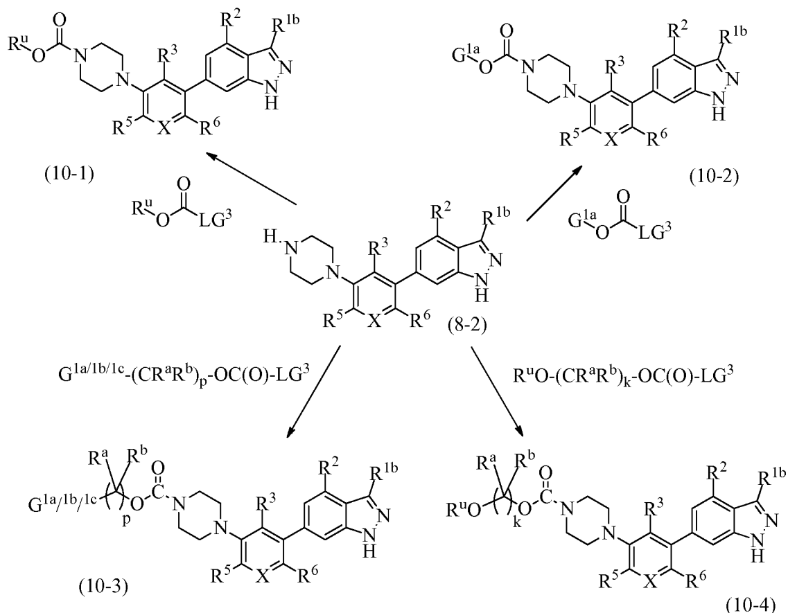
Scheme 10
