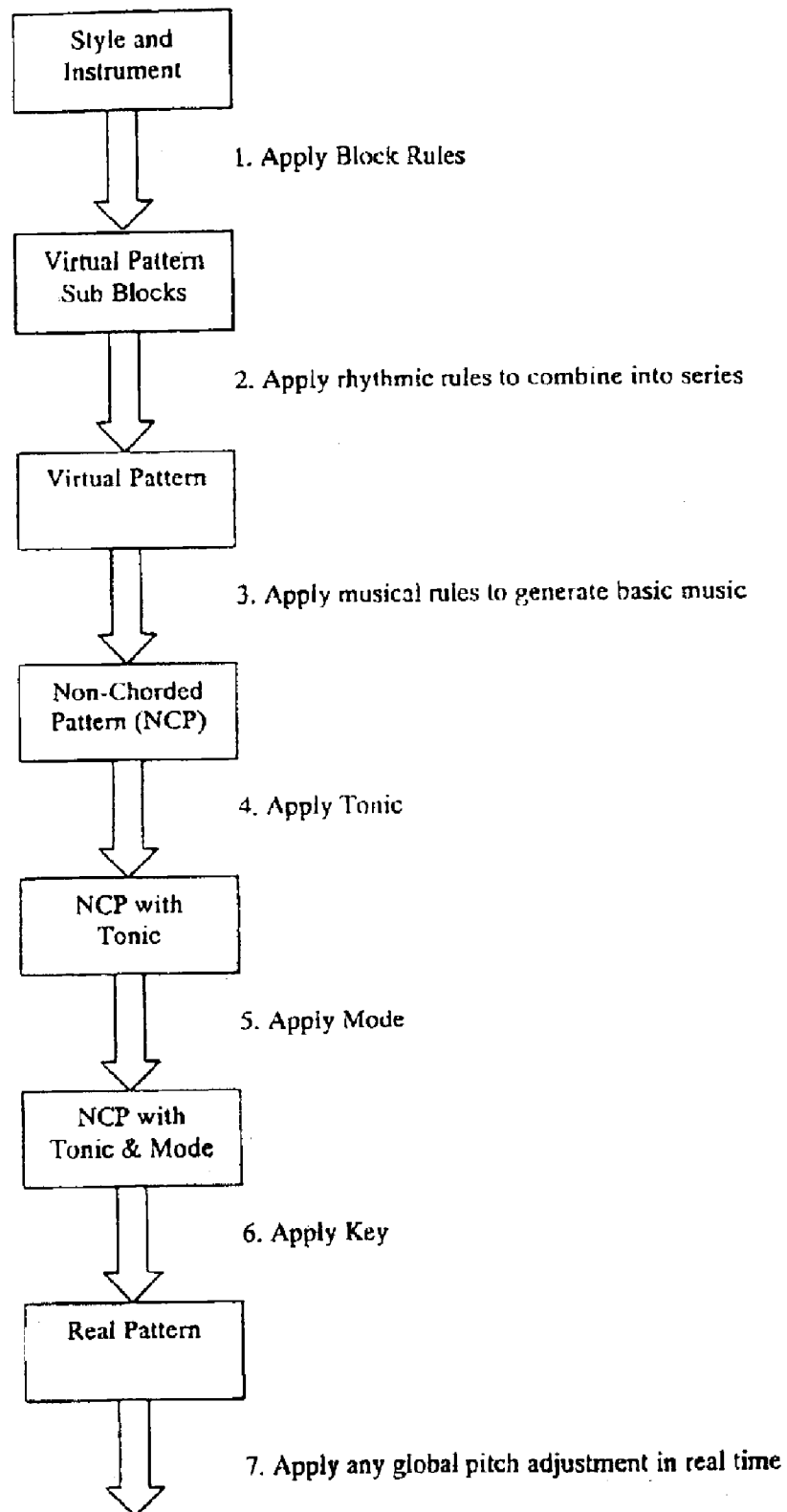
Figure 16 General Musical Generation Flow
