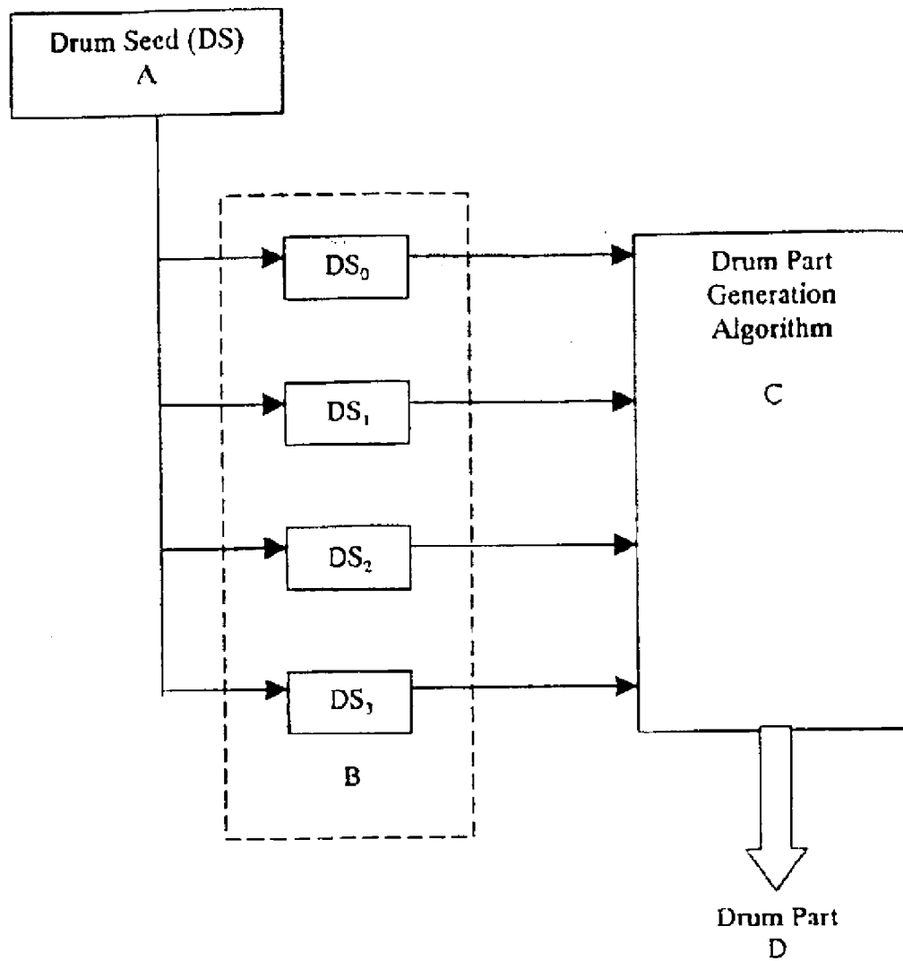
Figure 26 Pseudo-Random Number Implementation 1
