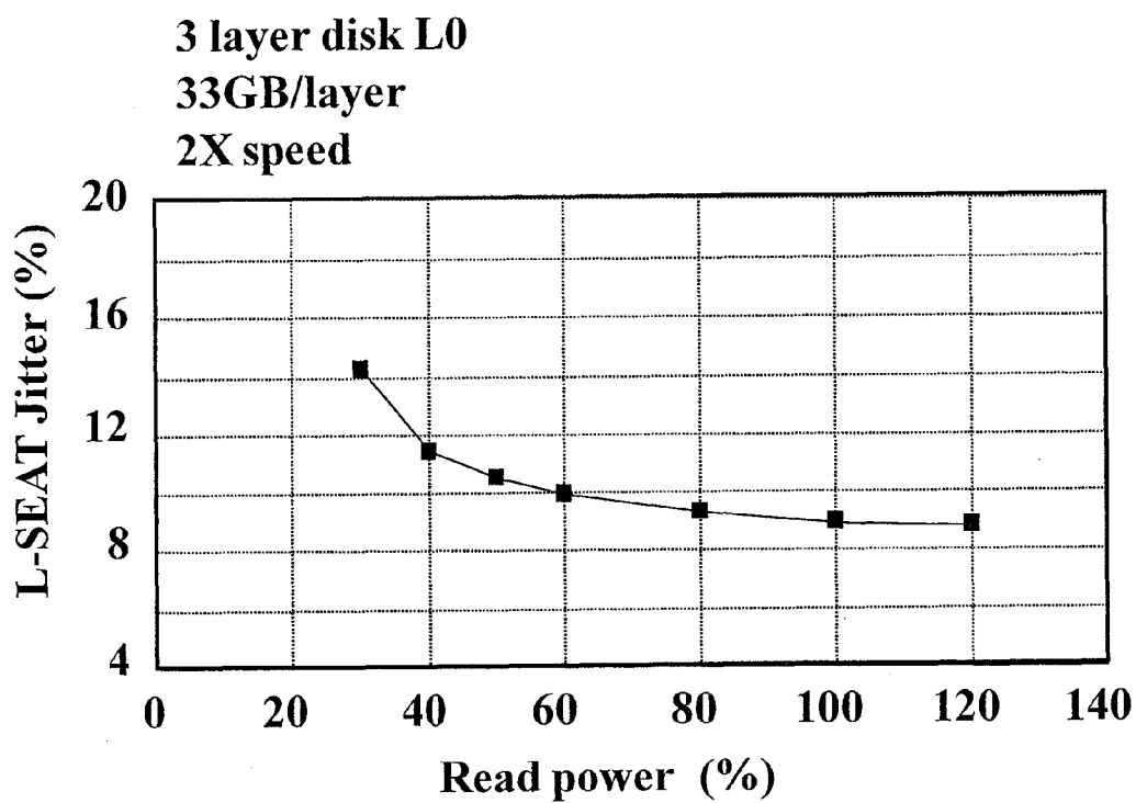
(a) Jitter
