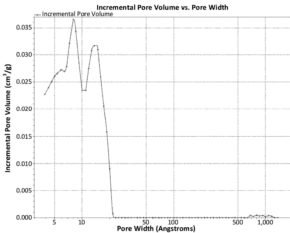
Figure 2. Pore distribution for carbon of Example 8.
