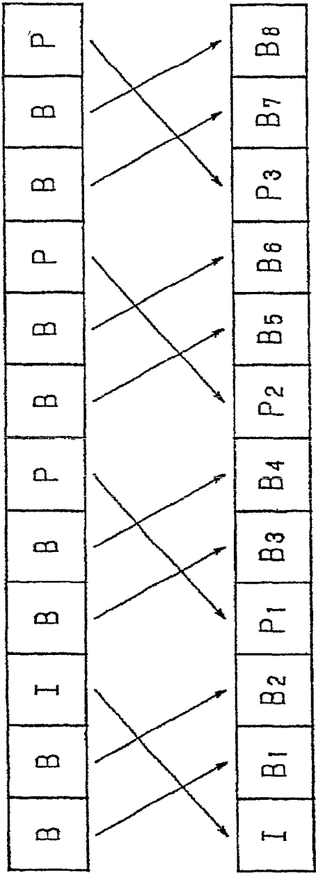
FIG. 7B PRIOR ART OUTPUT ORDER
