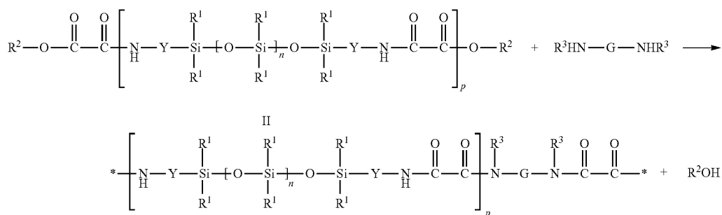
Reaction Scheme A
