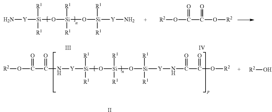
Reaction Scheme B
