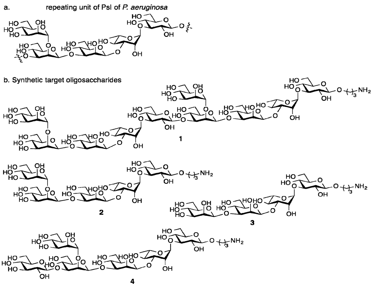
Figure 1. Structure of the repeating unit of the exopolysaccharide of P. aeruginosa and target compounds for chemical synthesis
