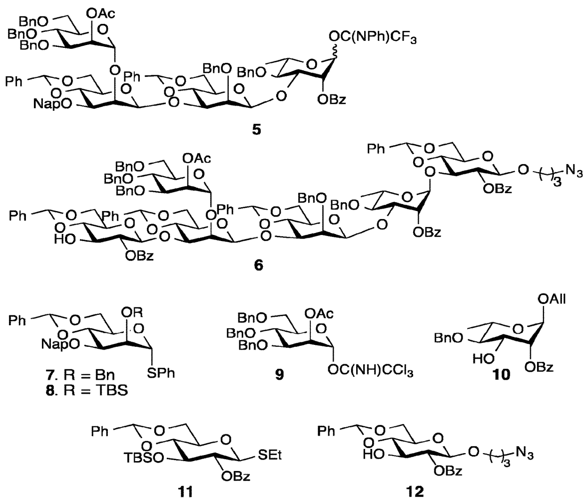
Figure 2. Building blocks for oligosaccharide assembly
