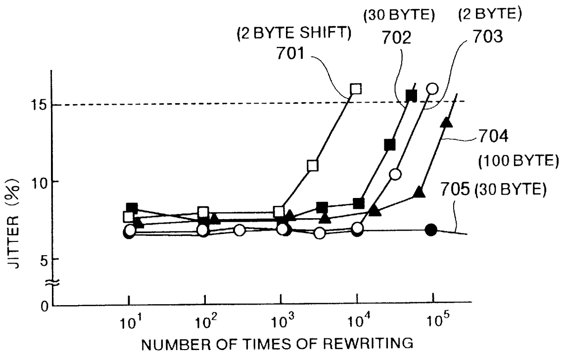
FIG.7 PRIOR ART
