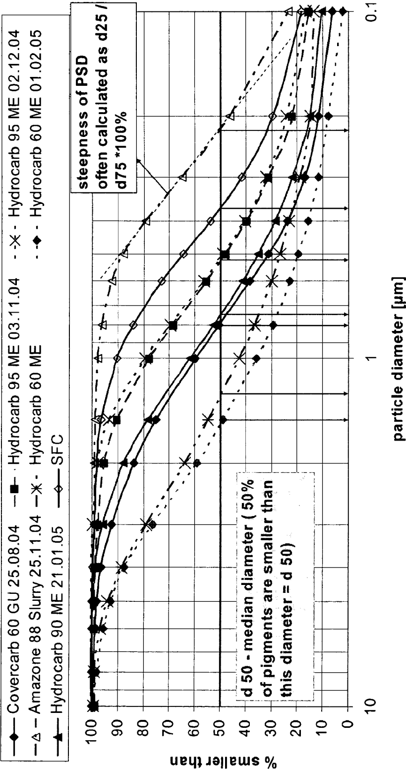
particle size distribution (PSD) of used pigments
