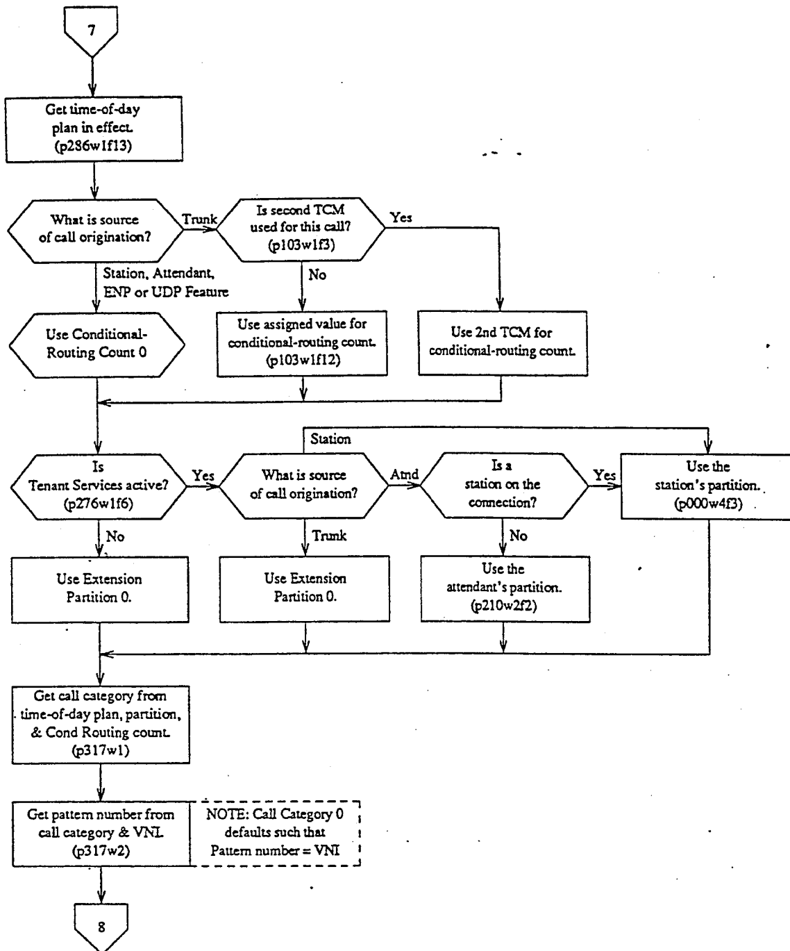
Figure 7. Pattern Selection
