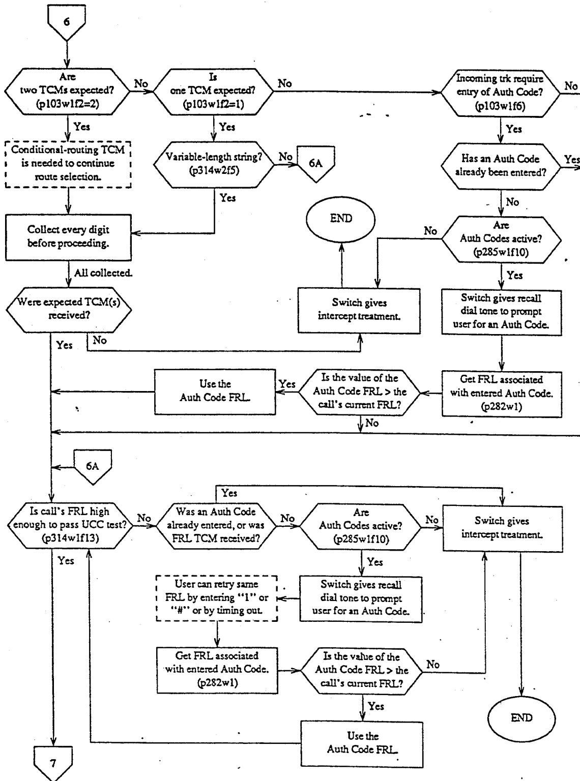
Figure 6. Check Permissions
