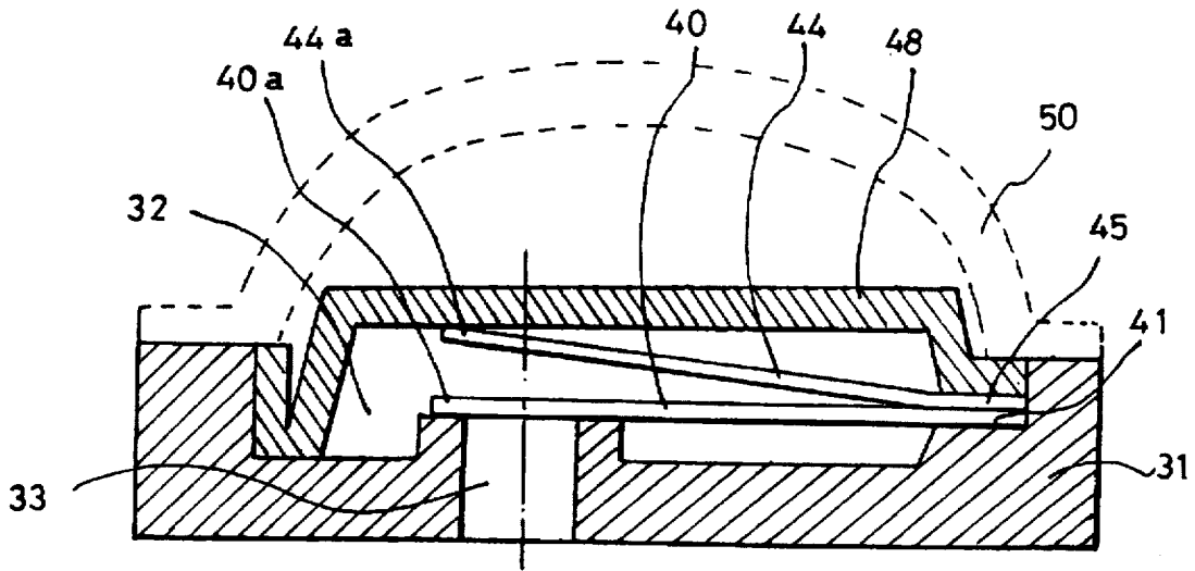
FIG. 5 CONVENTIONAL ART
