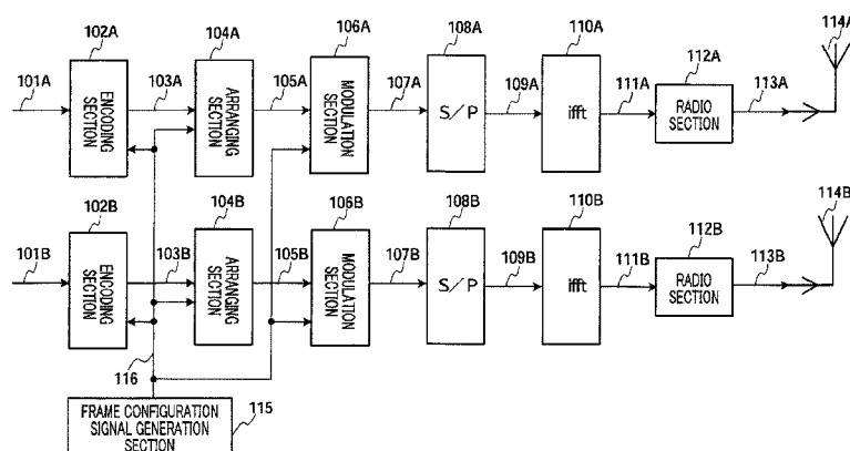
100 MULTI-ANTENNA TRANSMITTING APPARATUS
