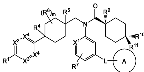
Formula (IIa).
