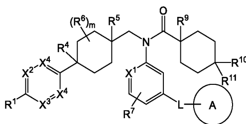
Formula (II);
