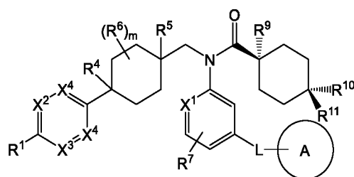
Formula (IIa).
