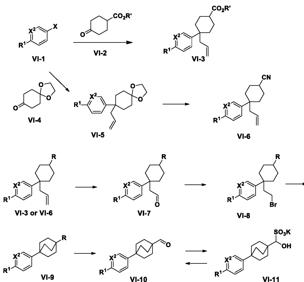
Scheme 6
