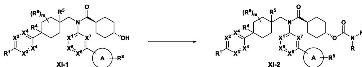
Scheme 11
