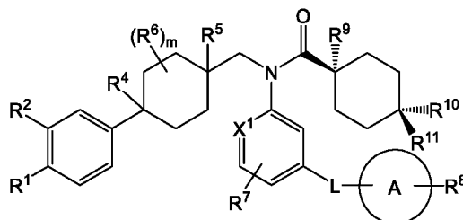
Formula (IIIa).
