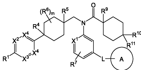
Formula (II);
