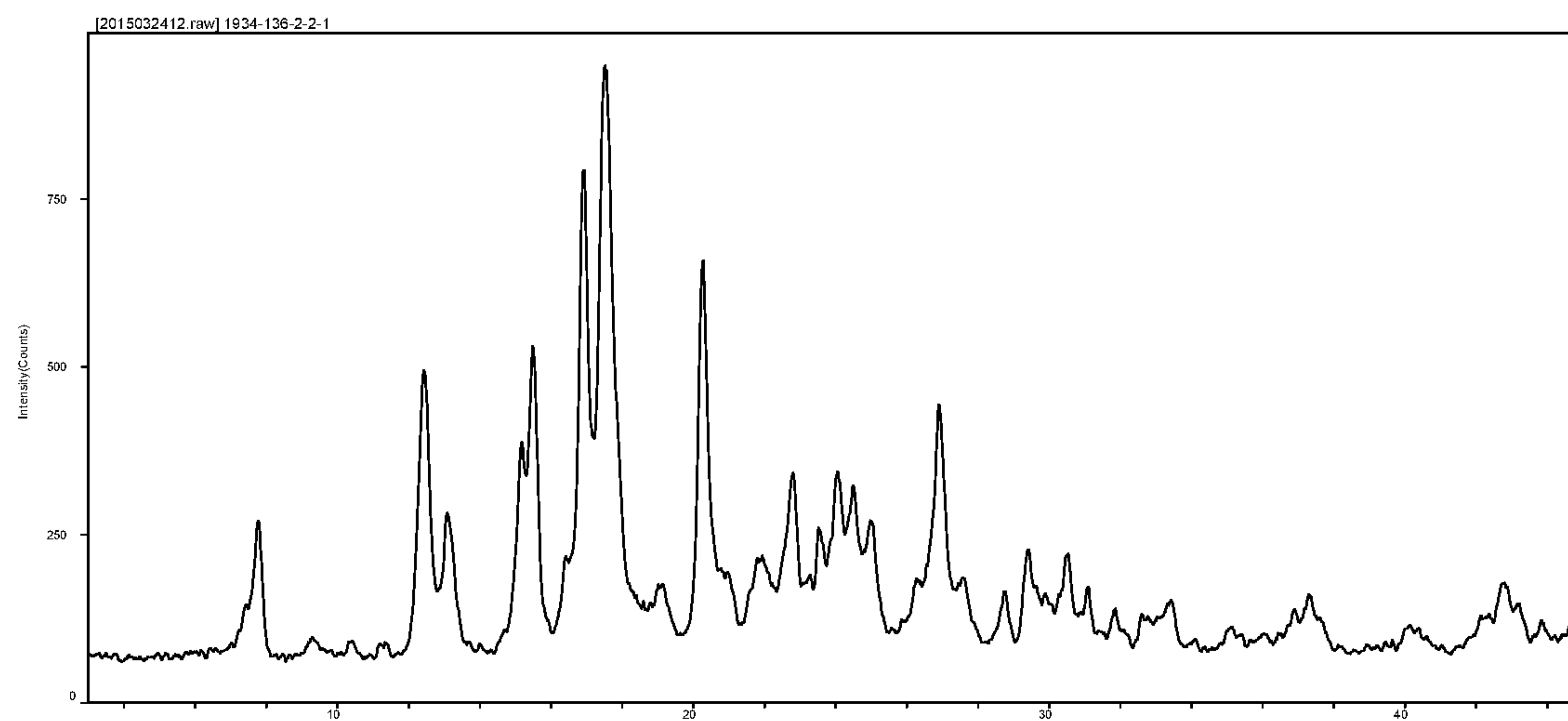
FIG. 8 XRPD Form III
