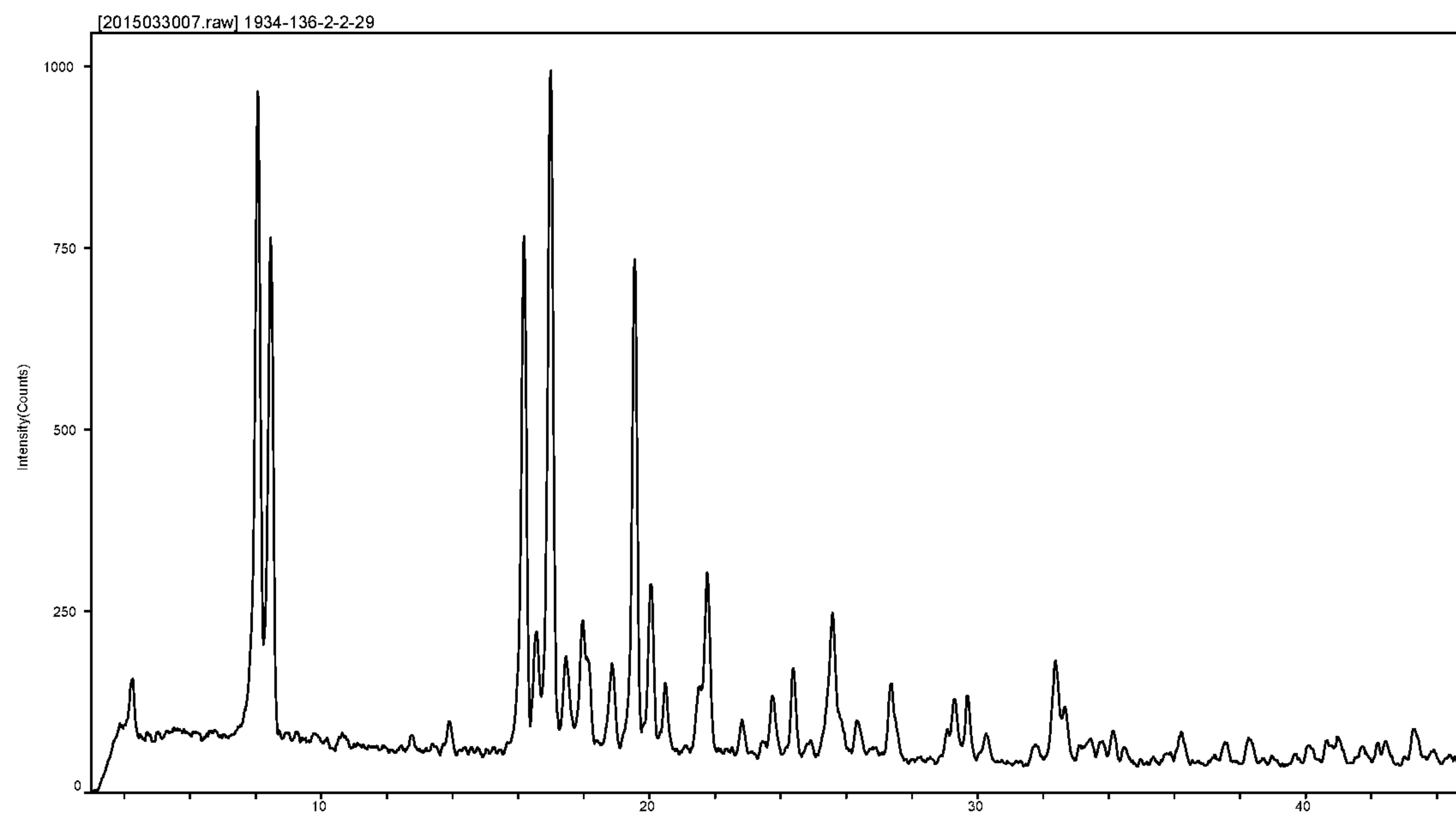
FIG. 14 XRPD Form VIII
