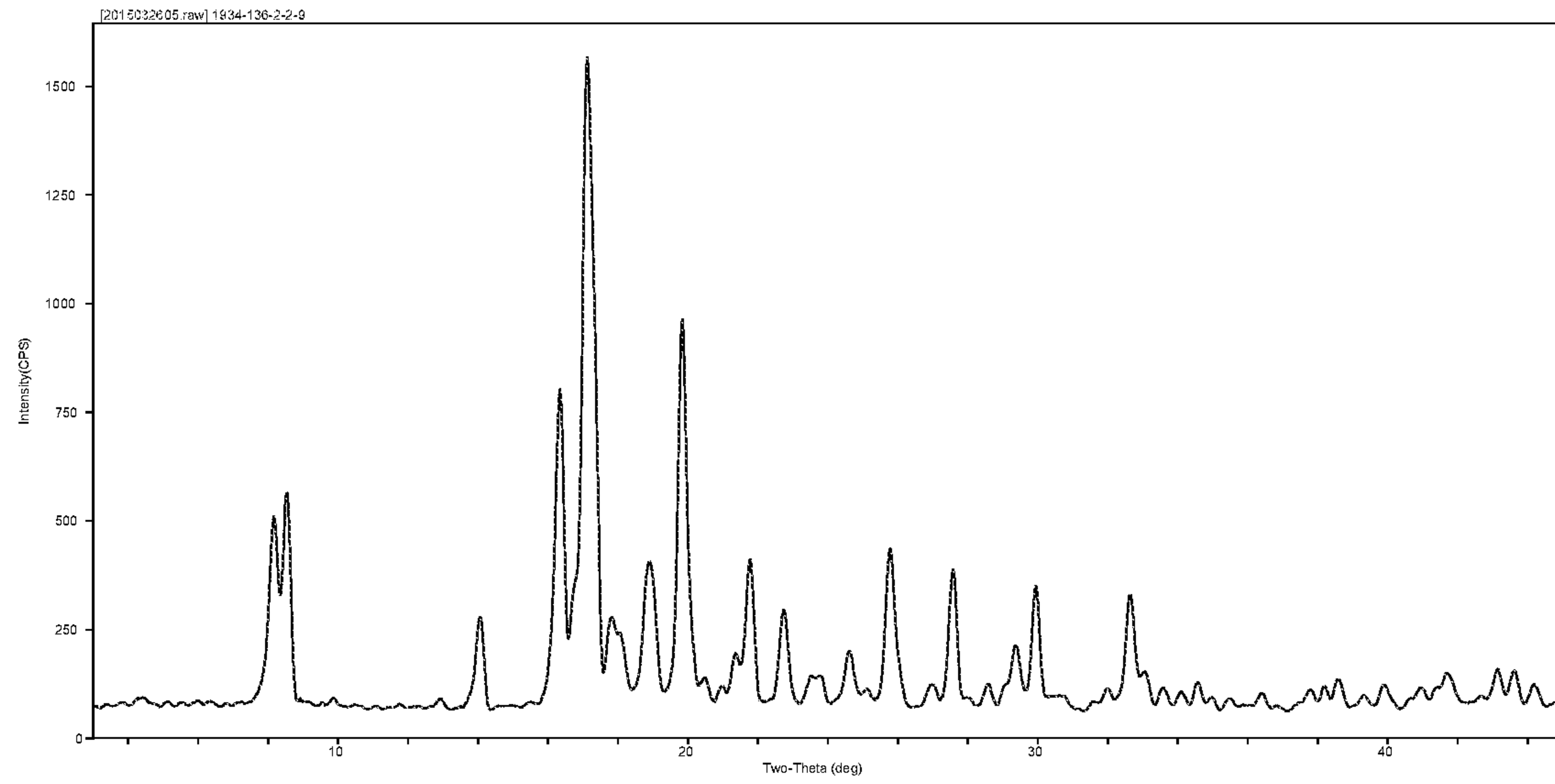
FIG. 10 XRPD Form V
