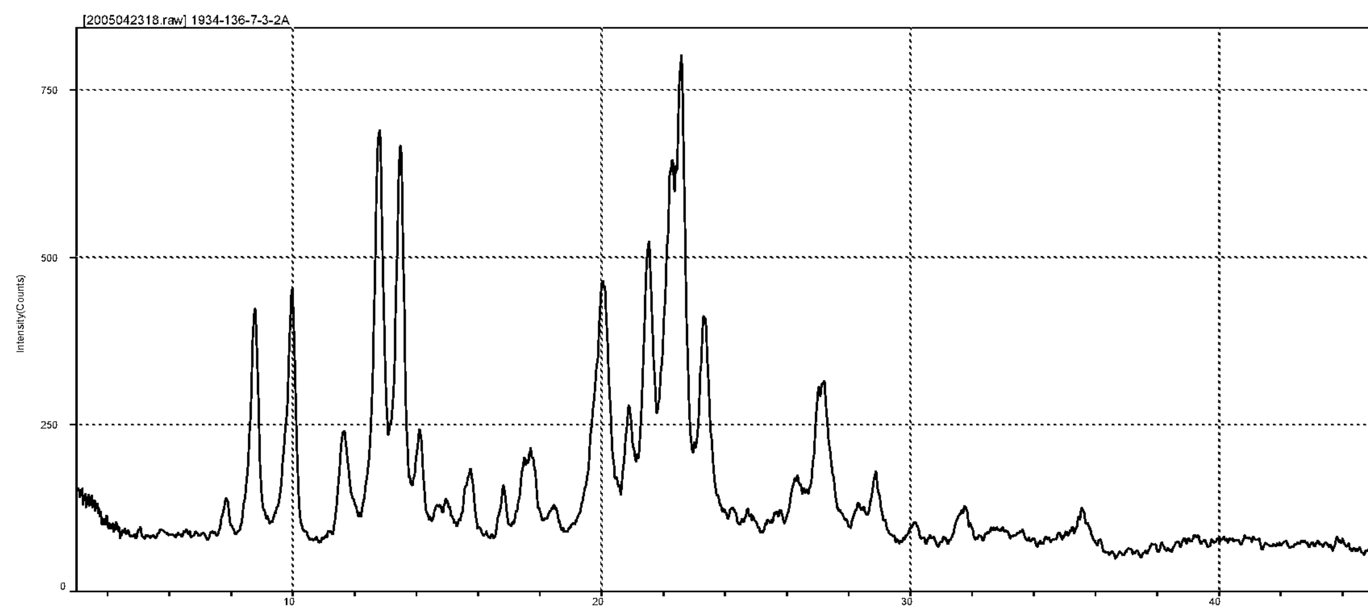
FIG. 7 XRPD Form Ia
