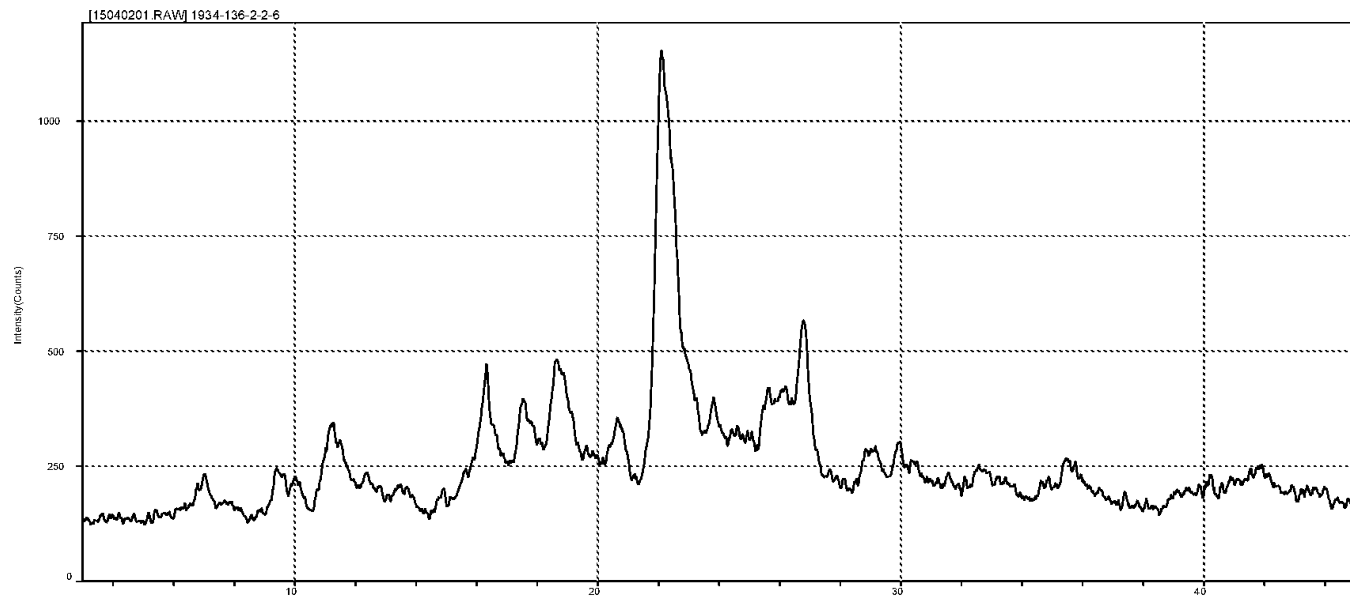
FIG. 9 XRPD Form IV
