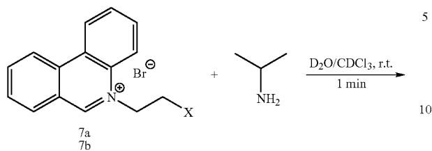
Scheme 2. NMR phase transfer experiment with the fluoro (7a) and hydroxy (7b) analogues of molecule 2.
