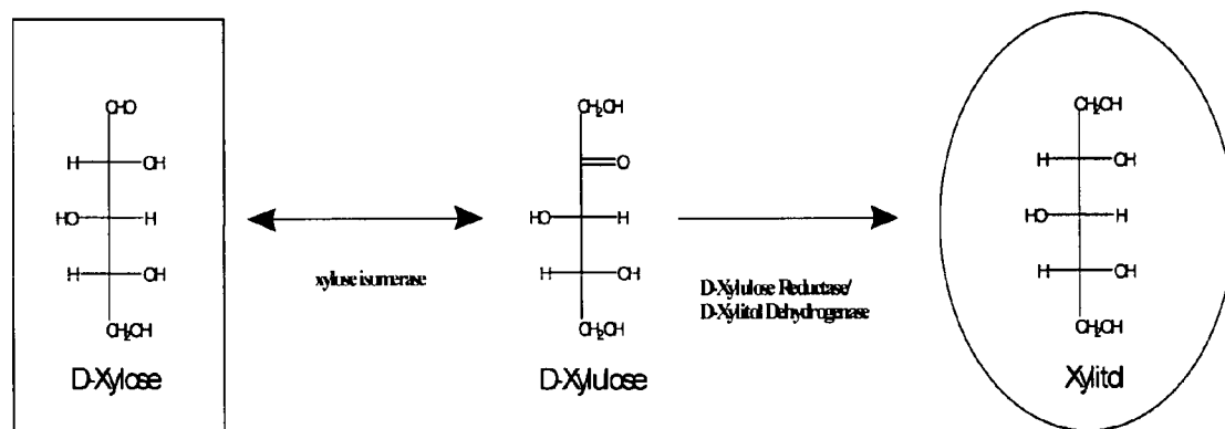
Figure 6. Alternative route to xylitol from D-xylose.
