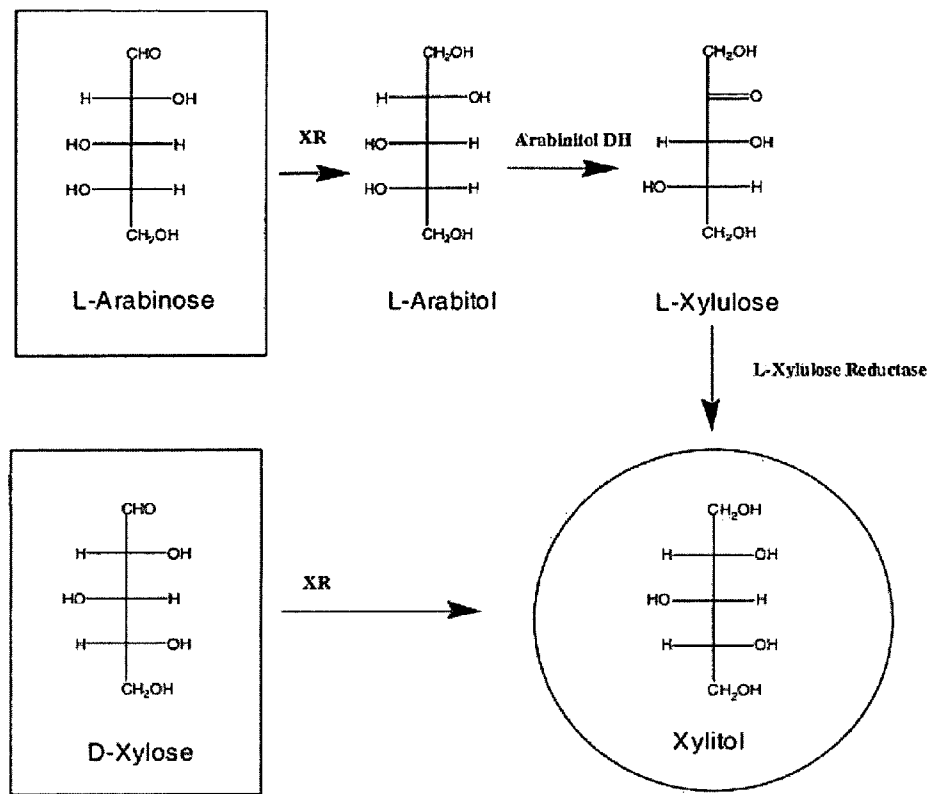
Figure 1. Xylitol synthesis from hemicellulose.
