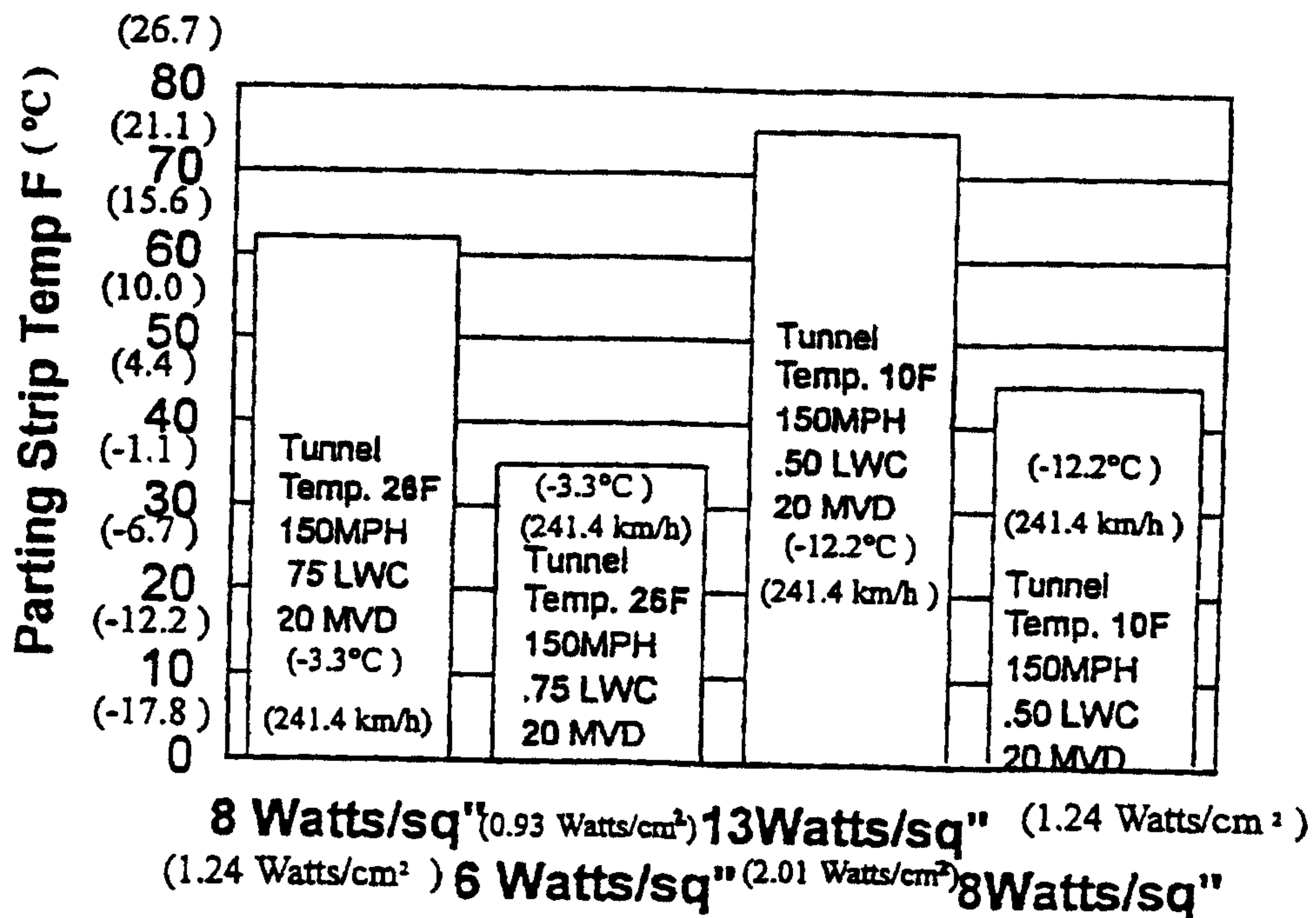
Power Requirements
