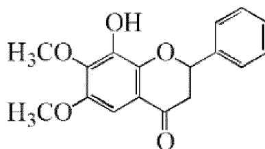
(I) 8-hydroxy-6,7-dimethoxyflavanone (Pa5)
