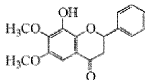
8-hydroxy-6,7-dimethoxyflavanone (Pa5)
