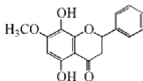
5,8-dihydroxy-7-methoxyflavanone (Pa5')
