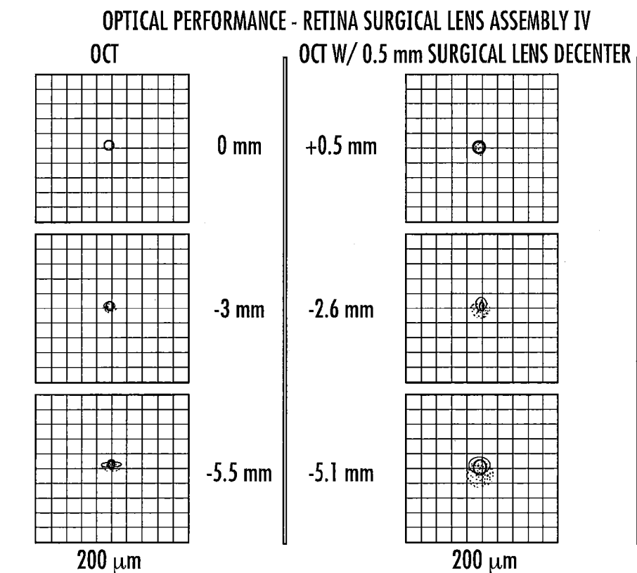
HIGH MAG. DOUBLET OPTICAL PERFORMANCE SUMMARY
