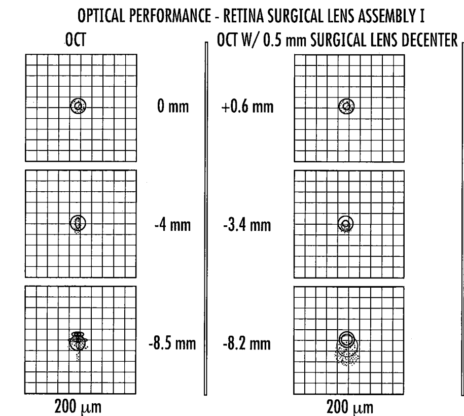
LOW MAG. SINGLET OPTICAL PERFORMANCE SUMMARY
