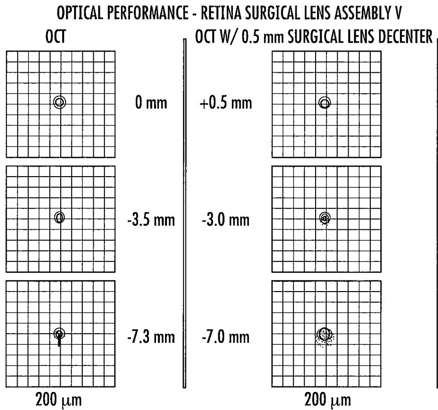
MID. MAG. DOUBLET OPTICAL PERFORMANCE SUMMARY
