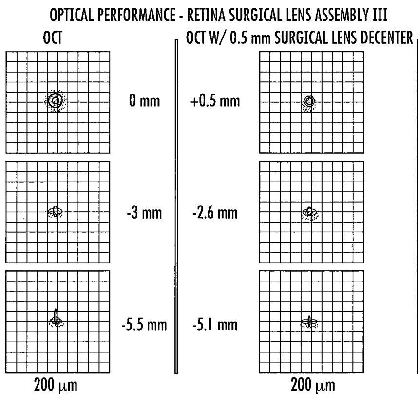
HIGH MAG. SINGLET OPTICAL PERFORMANCE SUMMARY
