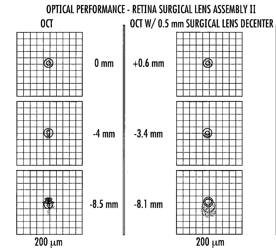
LOW MAG. SINGLET + DOUBLET OPTICAL PERFORMANCE SUMMARY
