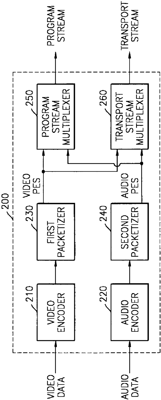
FIG. 2 (PRIOR ART)
