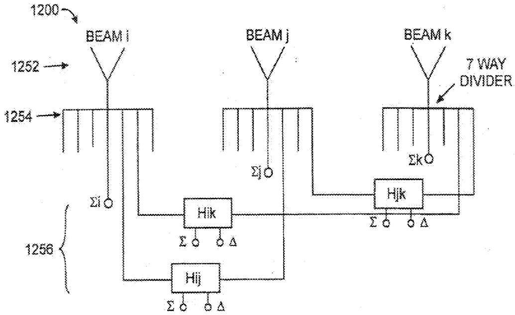
BEAM CIRCUITRY FIG. 12C
