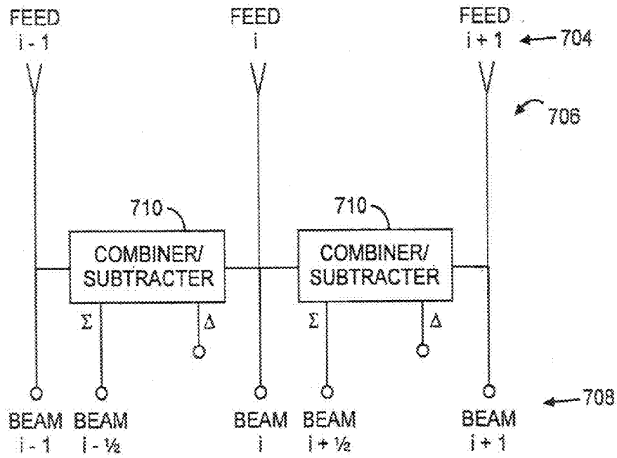
BEAM COMBINING CIRCUITRY FIG. 8
