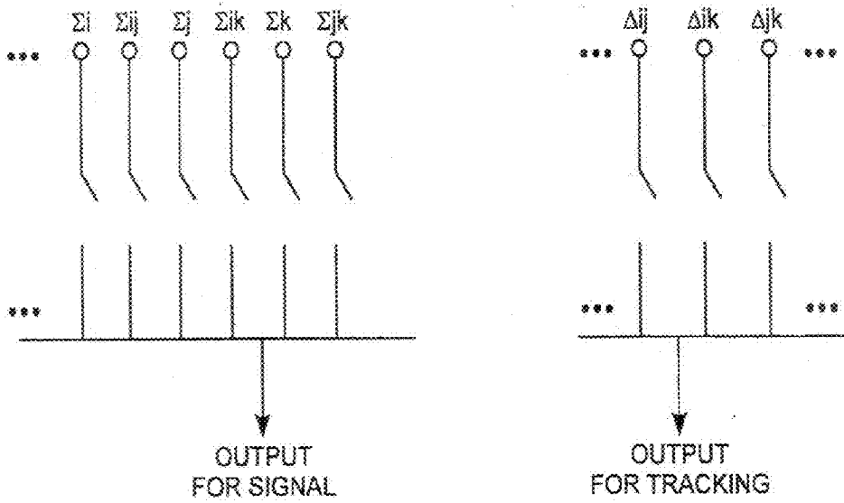
BEAM SELECTOR SWITCHES FIG. 12D
