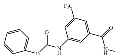
Phenyl 3-(methylcarbamoyl)-5-(trifluoromethyl) phenylcarbamate
