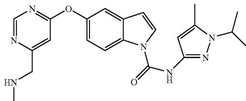
5-(6-Methylaminomethyl-pyrimidin-4-yloxy)-indole-1-carboxylic acid (1-isopropyl-5-methyl-1H-pyrazol-3-yl)-amide
