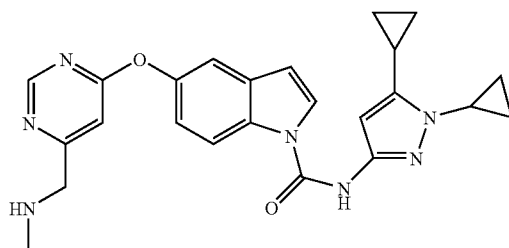
5-(6-Methylaminomethyl-pyrimidin-4-yloxy)-indole-1-carboxylic acid (1,5-dicyclopropyl-1H-pyrazol-3-yl)-amide
