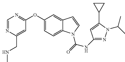
5-(6-Methylaminomethyl-pyrimidin-4-yloxy)-indole-1-carboxylic acid (5-cyclopropyl-1-isopropyl-1H-pyrazol-3-yl)-amide
