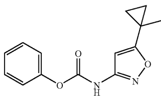
[5-(1-Methyl-cyclopropyl)-isoxazol-3-yl]-carbamic acid phenyl ester
