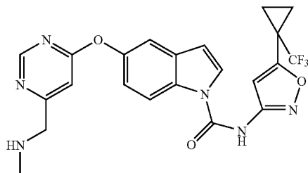
5-(6-Methylaminomethyl-pyrimidin-4-yloxy)-indole-1-carboxylic acid [5-(1-trifluoromethyl-cyclopropyl)-isoxazol-3-yl]-amide
