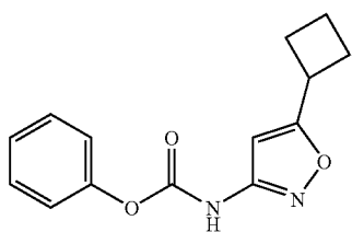
(5-Cyclobutyl-isoxazol-3-yl)-carbamic acid phenyl ester
