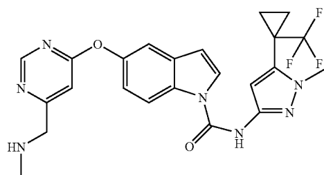
5-(6-Methylaminomethyl-pyrimidin-4-yloxy)-indole-1-carboxylic acid [1-methyl-5-(trifluoromethyl-cyclopropyl)-1H-pyrazol-3-yl]-amide
