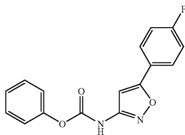
[5-(4-Fluoro-phenyl)-isoxazol-3-yl]-carbamic acid phenyl ester
