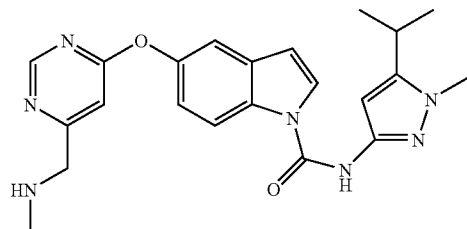
5-(6-Methylaminomethyl-pyrimidin-4-yloxy)-indole-1-carboxylic acid (5-isopropyl-1-methyl-1H-pyrazol-3-yl)-amide
