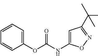
(3-tert-Butyl-isoxazol-5-yl)-carbamic acid phenyl ester
