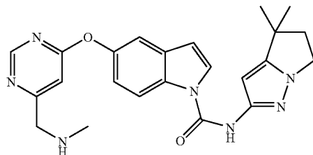
5-(6-Methylaminomethyl-pyrimidin-4-yloxy)-indole-1-carboxylic acid (4,4-dimethyl-5,6-dihydro-4H-pyrrolo[1,2-b]pyrazol-2-yl)-amide
