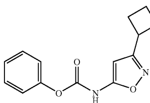
(3-Cyclobutyl-isoxazol-5-yl)-carbamic acid phenyl ester
