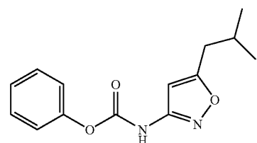
(5-Isobutyl-isoxazol-3-yl)-carbamic acid phenyl ester
