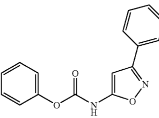
(3-Phenyl-isoxazol-5-yl)-carbamic acid phenyl ester
