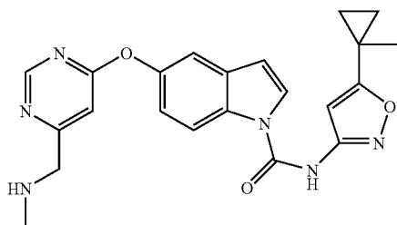
5-(6-Methylaminomethyl-pyrimidin-4-yloxy)-indole-1-carboxylic acid [5-(1-methyl cyclopropyl)-isoxazol-3-yl]-amide
