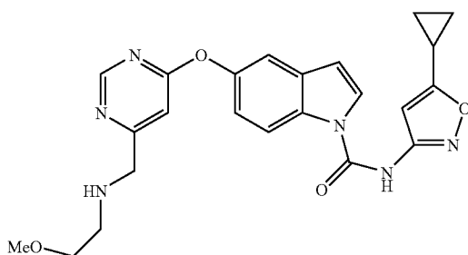
5-{6-[2-Methoxy-ethylamino)-methyl]-pyrimidin-4-yloxy}-indole-1-carboxylic acid (5-cyclopropyl-isoxazol-3-yl)-amide
