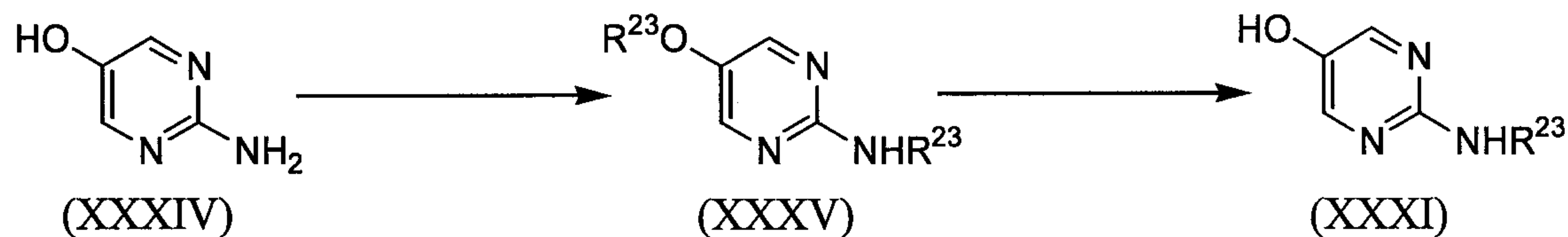
Reaction scheme 8
