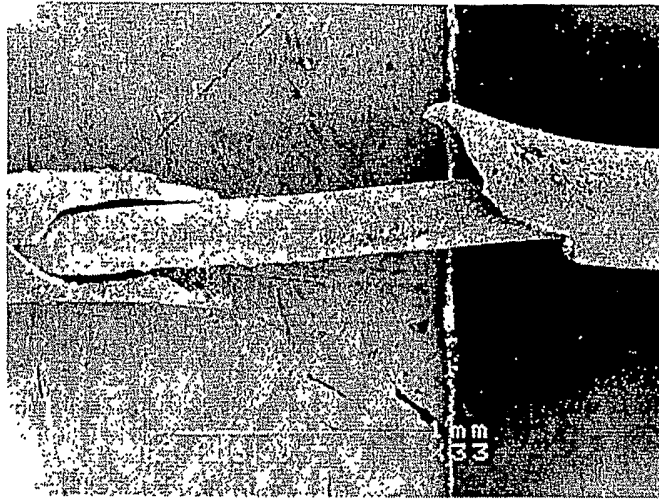
Figure 4. Copper wire after oxidation in air at 700 °C.
