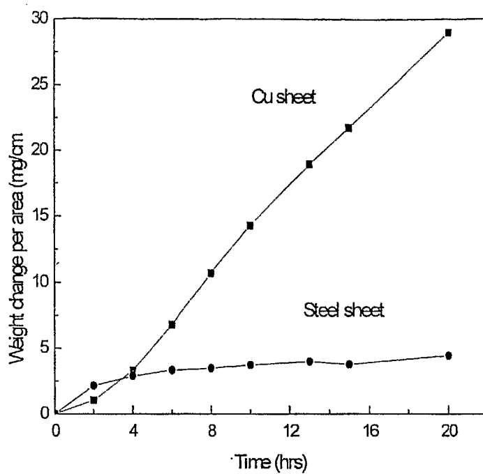
Figure 3. Weight change of copper and steel during oxidation in air at 500 °C under thermal cycle.
