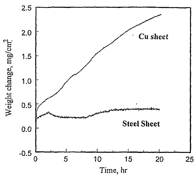
Figure 1. Weight change during the oxidation of steel and copper in 40%O 2 /Ar at 500 °C.
