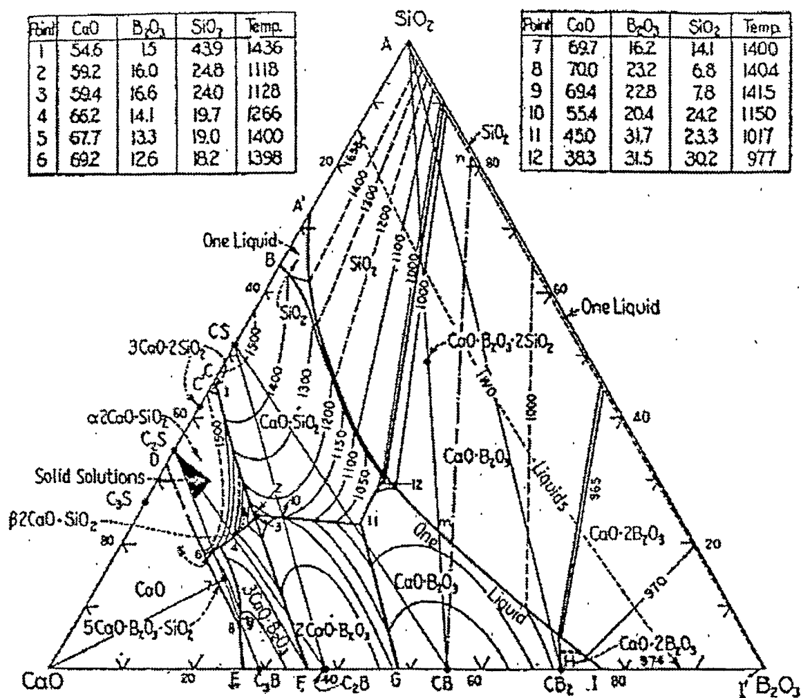
Figure 5. CaO-SiO 2 -B 2 O 3 phase diagram.
