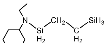
1-cyclohexylethylamino-1,4- disilabutane
