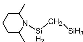
1-2,6-dimethylpiperidino- 1,3-disilapropane
