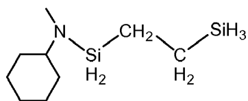
1-cyclohexylmethylamino- 1,4-disilabutane
