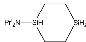
1-di-iso-propylamino-1,4-disilacyclohexane
