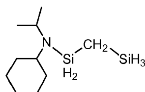
1-cyclohexyl-iso- propylamino-1,3- disilapropane
