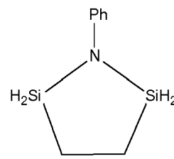
1-phenyl-1-aza-2,5-disilacyclopentane
