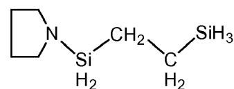
1-pyrrolidino-1,4-disilabutane
