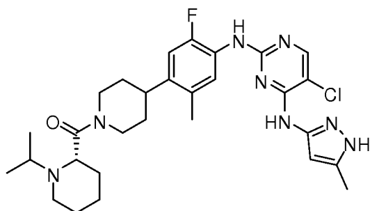
(S)-(4-(4-(5-chloro-4-(5-methyl-1H-pyrazol-3-ylamino)pyrimidin-2-ylamino)-5-fluoro-2-methylphenyl)piperidin-1-yl)(1-isopropylpiperidin-2-yl)methanone
