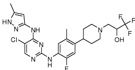
3-(4-(4-(5-chloro-4-(5-methyl-1H-pyrazol-3-ylamino) pyrimidin-2-ylamino)-5-fluoro-2-methylphenyl) piperidin-1-yl)-1,1,1-trifluoropropan-2-ol
