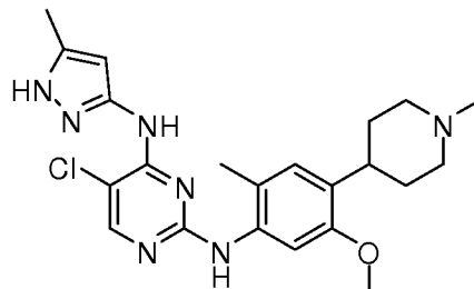
5-chloro-N2-(5-methoxy-2-methyl-4-(1-methylpiperidin-4-yl)phenyl)-N4-(5-methyl-1H-pyrazol-3-yl)pyrimidine-2,4-diamine
