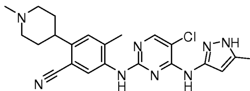
5-(5-chloro-4-(5-methyl-1H-pyrazol-3-ylamino)pyrimidin-2-ylamino)-4-methyl-2-(1-methylpiperidin-4-yl)benzonitrile
