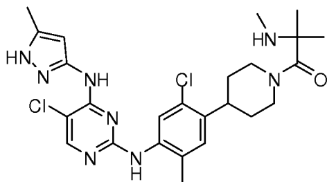
1-(4-(2-chloro-4-(5-chloro-4-(5-methyl-1H-pyrazol-3-ylamino)pyrimidin-2-ylamino)-5-methylphenyl)piperidin-1-yl)-2-methyl-2-(methylamino)propan-1-one
