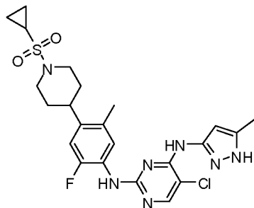
5-chloro-N2-(4-(1-(cyclopropylsulfonyl)piperidin-4-yl)-2-fluoro-5-methylphenyl)-N4-(5-methyl-1H-pyrazol-3-yl)pyrimidine-2,4-diamine
