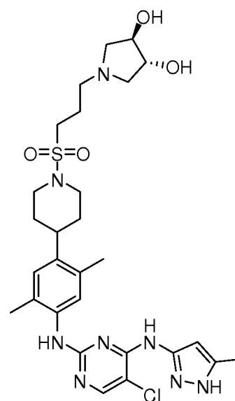
(3R,4R)-1-(3-(4-(4-(5-chloro-4-(5-methyl-1H-pyrazol-3-ylamino)pyrimidin-2-ylamino)-2,5-dimethylphenyl)piperidin-1-ylsulfonyl)propyl)pyrrolidine-3,4-diol
