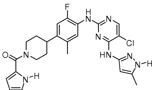
(4-(4-(5-chloro-4-(5-methyl-1H-pyrazol-3-ylamino)pyrimidin-2-ylamino)-5-fluoro-2-methylphenyl)piperidin-1-yl)(1H-pyrrol-2-yl)methanone
