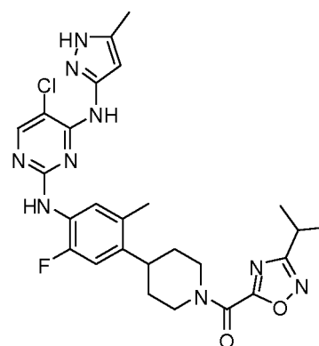
(4-(4-(5-chloro-4-(5-methyl-1H-pyrazol-3-ylamino)pyrimidin-2-ylamino)-5-fluoro-2-methylphenyl)piperidin-1-yl)(3-isopropyl-1,2,4-oxadiazol-5-yl)methanone
