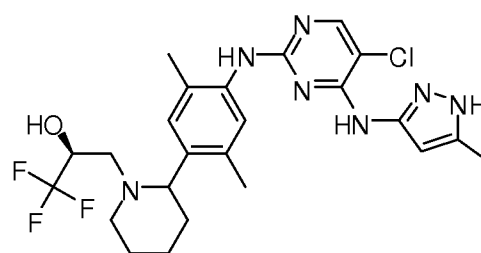
(2S)-3-(2-(4-(5-chloro-4-(5-methyl-1H-pyrazol-3-ylamino)pyrimidin-2-ylamino)-2,5-dimethylphenyl)piperidin-1-yl)-1,1,1-trifluoropropan-2-ol
