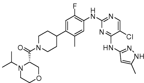
(S)-(4-(4-(5-chloro-4-(5-methyl-1H-pyrazol-3-ylamino)pyrimidin-2-ylamino)-5-fluoro-2-methylphenyl)piperidin-1-yl)(4-isopropylmorpholin-3-yl)methanone
