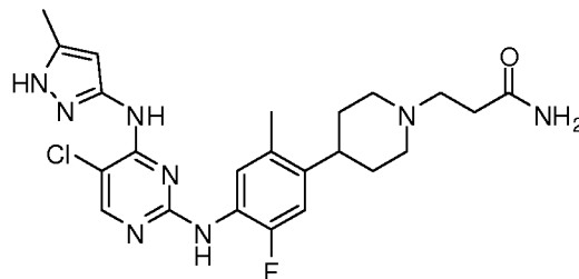
3-(4-(4-(5-chloro-4-(5-methyl-1H-pyrazol-3-ylamino)pyrimidin-2-ylamino)-5-fluoro-2-methylphenyl)piperidin-1-yl)propanamide
