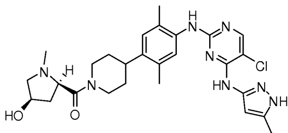
(4-(4-(5-chloro-4-(5-methyl-1H-pyrazol-3-ylamino)pyrimidin-2-ylamino)-2,5-dimethylphenyl)piperidin-1-yl)((2R,4R)-4-hydroxy-1-methylpyrrolidin-2-yl)methanone
