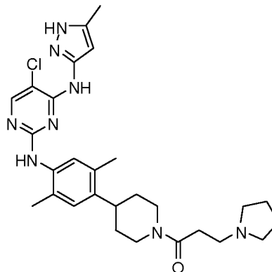
1-(4-(4-(5-chloro-4-(5-methyl-1H-pyrazol-3-ylamino)pyrimidin-2-ylamino)-2,5-dimethylphenyl)piperidin-1-yl)-3-(pyrrolidin-1-yl)propan-1-one
