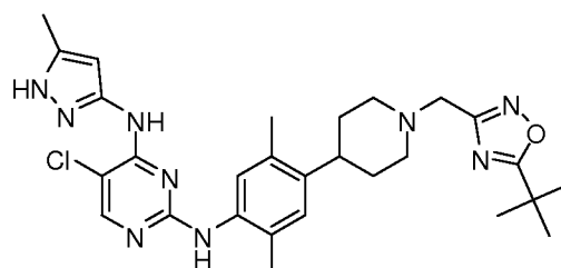
N2-(4-(1-((5-tert-butyl-1,2,4-oxadiazol-3-yl)methyl)piperidin-4-yl)-2,5-dimethylphenyl)-5-chloro-N4-(5-methyl-1H-pyrazol-3-yl)pyrimidine-2,4-diamine
