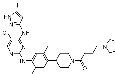
1-(4-(4-(5-chloro-4-(5-methyl-1H-pyrazol-3-ylamino)pyrimidin-2-ylamino)-2,5-dimethylphenyl)piperidin-1-yl)-4-(pyrrolidin-1-yl)butan-1-one
