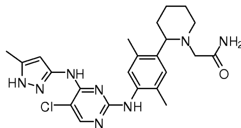
2-(2-(4-(5-chloro-4-(5-methyl-1H-pyrazol-3-ylamino)pyrimidin-2-ylamino)-2,5-dimethylphenyl)piperidin-1-yl)acetamide
