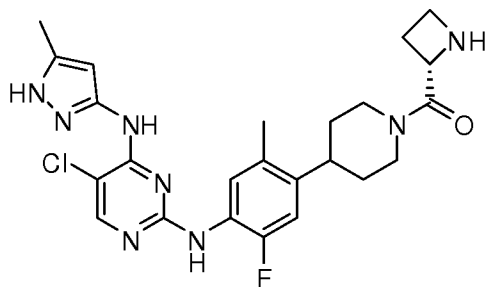
(S)-azetidin-2-yl(4-(4-(5-chloro-4-(5-methyl-1H-pyrazol-3-ylamino)pyrimidin-2-ylamino)-5-fluoro-2-methylphenyl)piperidin-1-yl)methanone
