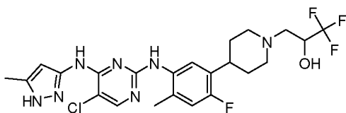
3-(4-(5-(5-chloro-4-(5-methyl-1H-pyrazol-3-ylamino)pyrimidin-2-ylamino)-2-fluoro-4-methylphenyl)piperidin-1-yl)-1,1,1-trifluoropropan-2-ol
