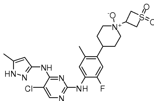
5-Chloro-N2-{4-[1-(1,1-dioxo-1λ6-thietan-3-yl)-1-oxide-piperidin-4-yl]-2-fluoro-5-methyl-phenyl}-N4-(5-ethyl-1H-pyrazol-3-yl)-pyrimidine-2,4-diamine
