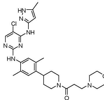
1-(4-(4-(5-chloro-4-(5-methyl-1H-pyrazol-3-ylamino)pyrimidin-2-ylamino)-2,5-dimethylphenyl)piperidin-1-yl)-3-morpholinopropan-1-one
