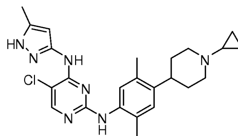
5-chloro-N2-(4-(1-cyclopropyl)piperidin-4-yl)-2,5-dimethylphenyl)-N4-(5-methyl-1H-pyrazol-3-yl)pyrimidine-2,4-diamine
