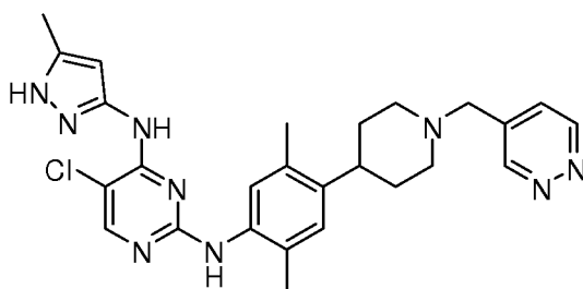
5-chloro-N2-(2,5-dimethyl-4-(1-(pyridazin-4-ylmethyl)piperidin-4-yl)phenyl)-N4-(5-methyl-1H-pyrazol-3-yl)pyrimidine-2,4-diamine
