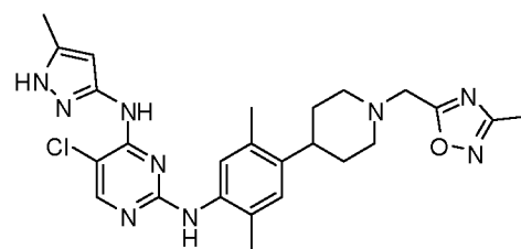
5-chloro-N2-(2,5-dimethyl-4-(1-((3-methyl-1,2,4-oxadiazol-5-yl)methyl)piperidin-4-yl)phenyl)-N4-(5-methyl-1H-pyrazol-3-yl)pyrimidine-2,4-diamine
