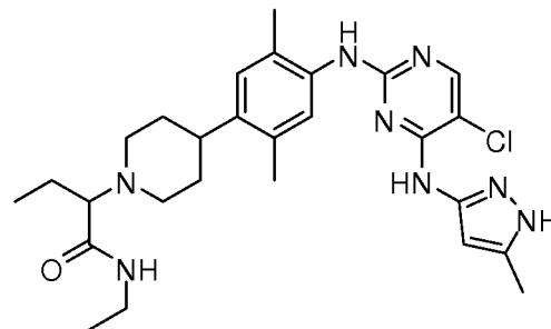
2-(4-(4-(5-chloro-4-(5-methyl-1H-pyrazol-3-ylamino)pyrimidin-2-ylamino)-2,5-dimethylphenyl)piperidin-1-yl)-N-ethylbutanamide
