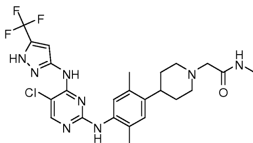
2-(4-(4-(5-chloro-4-(5-(trifluoromethyl)-1H-pyrazol-3-ylamino)pyrimidin-2-ylamino)-2,5-dimethylphenyl)piperidin-1-yl)-N-methylacetamide
