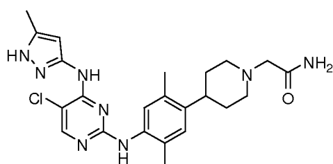
2-(4-(4-(5-chloro-4-(5-methyl-1H-pyrazol-3-ylamino)pyrimidin-2-ylamino)-2,5-dimethylphenyl)piperidin-1-yl)acetamide
