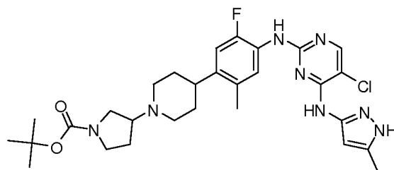
tert-butyl 3-(4-(4-(5-chloro-4-(5-methyl-1H-pyrazol-3-ylamino)pyrimidin-2-ylamino)-5-fluoro-2-methylphenyl)piperidin-1-yl)pyrrolidine-1-carboxylate
