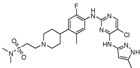
2-(4-(4-(5-chloro-4-(5-methyl-1H-pyrazol-3-ylamino)pyrimidin-2-ylamino)-5-fluoro-2-methylphenyl)piperidin-1-yl)-N,N-dimethylethanesulfonamide
