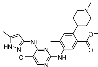
methyl 5-(5-chloro-4-(5-methyl-1H-pyrazol-3-ylamino)pyrimidin-2-ylamino)-4-methyl-2-(1-methylpiperidin-4-yl)benzoate
