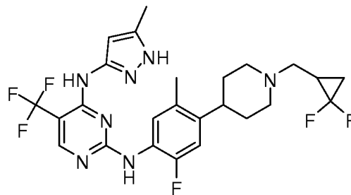
N2-(4-(1-((2,2-difluorocyclopropyl)methyl)piperidin-4-yl)-2-fluoro-5-methylphenyl)-N4-(5-methyl-1H-pyrazol-3-yl)-5-(trifluoromethyl)pyrimidine-2,4-diamine
