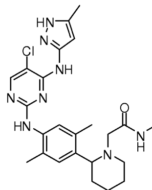
2-(2-(4-(5-chloro-4-(5-methyl-1H-pyrazol-3-ylamino)pyrimidin-2-ylamino)-2,5-dimethylphenyl)piperidin-1-yl)-N-methylacetamide
