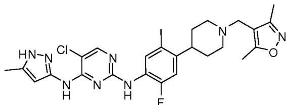
5-Chloro-N2-(4-(1-((3,5-dimethylisoxazol-4-yl)methyl)piperidin-4-yl)-2-fluoro-5-methylphenyl)-N4-(5-methyl-1H-pyrazol-3-yl)pyrimidine-2,4-diamine
