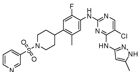
5-chloro-N2-(2-fluoro-5-methyl-4-(1-(pyridin-3-ylsulfonyl)piperidin-4-yl)phenyl)-N4-(5-methyl-1H-pyrazol-3-yl)pyrimidine-2,4-diamine
