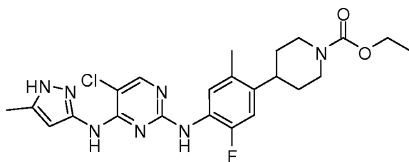
Ethyl 4-(4-(5-chloro-4-(5-methyl-1H-pyrazol-3-ylamino)pyrimidin-2-ylamino)-5-fluoro-2-methylphenyl)piperidine-1-carboxylate
