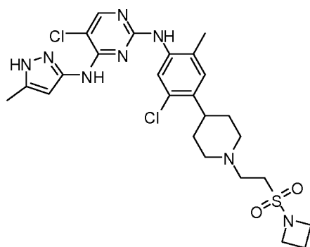
N2-(4-(1-(2-(azetidin-1-ylsulfonyl)ethyl)piperidin-4-yl)-5-chloro-2-methylphenyl)-5-chloro-N4-(5-methyl-1H-pyrazol-3-yl)pyrimidine-2,4-diamine
