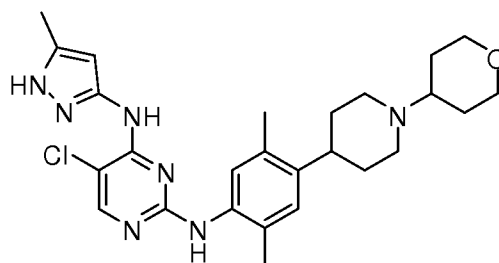
5-chloro-N2-(2,5-dimethyl-4-(1-(tetrahydro-2H-pyran-4-yl)piperidin-4-yl)phenyl)-N4-(5-methyl-1H-pyrazol-3-yl)pyrimidine-2,4-diamine
