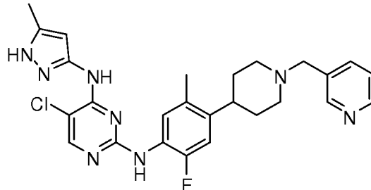
5-chloro-N2-(2-fluoro-5-methyl-4-(1-(pyridin-3-ylmethyl)piperidin-4-yl)phenyl)-N4-(5-methyl-1H-pyrazol-3-yl)-pyrimidine-2,4-diamine
