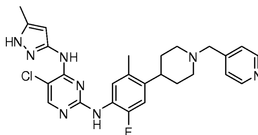
5-chloro-N2-(2-fluoro-5-methyl-4-(1-(pyridin-4-ylmethyl)piperidin-4-yl)phenyl)-N4-(5-methyl-1H-pyrazol-3-yl)pyrimidine-2,4-diamine
