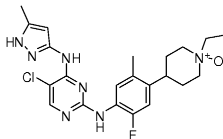
4-(4-(5-chloro-4-(5-methyl-1H-pyrazol-3-ylamino)pyrimidin-2-ylamino)-5-fluoro-2-methylphenyl)-1-ethylpiperidine 1-oxide
