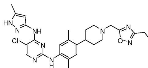
5-chloro-N2-(4-(1-((3-ethyl-1,2,4-oxadiazol-5-yl)methyl)piperidin-4-yl)-2,5-dimethylphenyl)-N4-(5-methyl-1H-pyrazol-3-yl)pyrimidine-2,4-diamine
