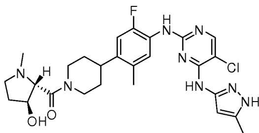
(4-(4-(5-chloro-4-(5-methyl-1H-pyrazol-3-ylamino)pyrimidin-2-ylamino)-5-fluoro-2-methylphenyl)piperidin-1-yl)((2S,3R)-3-hydroxy-1-methylpyrrolidin-2-yl)methanone
