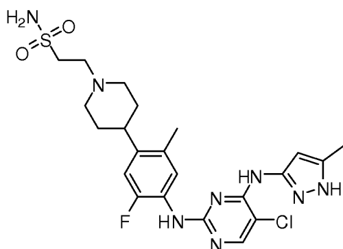
2-(4-(4-(5-chloro-4-(5-methyl-1H-pyrazol-3-ylamino)pyrimidin-2-ylamino)-5-fluoro-2-methylphenyl)piperidin-1-yl)ethanesulfonamide
