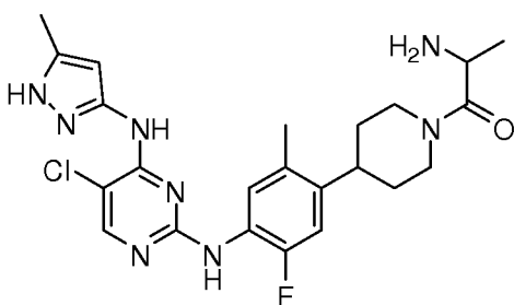
2-amino-1-(4-(4-(5-chloro-4-(5-methyl-1H-pyrazol-3-ylamino)pyrimidin-2-ylamino)-5-fluoro-2-methylphenyl)piperidin-1-yl)propan-1-one
