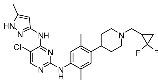
5-chloro-N2-(4-(1-((2,2-difluorocyclopropyl)methyl)piperidin-4-yl)-2,5-dimethylphenyl)-N4-(5-methyl-1H-pyrazol-3-yl)pyrimidine-2,4-diamine
