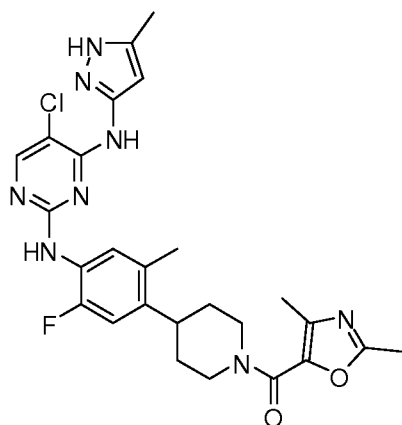
(4-(4-(5-chloro-4-(5-methyl-1H-pyrazol-3-ylamino)pyrimidin-2-ylamino)-5-fluoro-2-methylphenyl)piperidin-1-yl)(2,4-dimethyloxazol-5-yl)methanone
