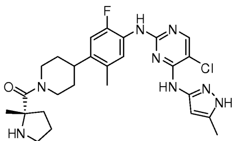
(S)-(4-(4-(5-chloro-4-(5-methyl-1H-pyrazol-3-ylamino)pyrimidin-2-ylamino)-5-fluoro-2-methylphenyl)piperidin-1-yl)(2-methylpyrrolidin-2-yl)methanone
