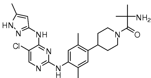
2-amino-1-(4-(4-(5-chloro-4-(5-methyl-1H-pyrazol-3-ylamino)pyrimidin-2-ylamino)-2,5-dimethylphenyl)piperidin-1-yl)-2-methylpropan-1-one
