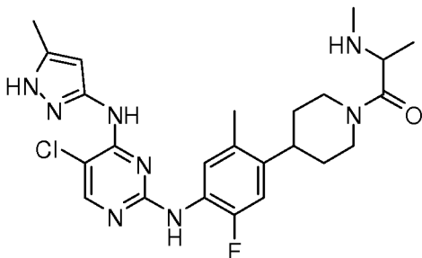
1-(4-(4-(5-chloro-4-(5-methyl-1H-pyrazol-3-ylamino)pyrimidin-2-ylamino)-5-fluoro-2-methylphenyl)piperidin-1-yl)-2-(methylamino)propan-1-one
