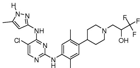
3-(4-(4-(5-chloro-4-(5-methyl-1H-pyrazol-3-ylamino)pyrimidin-2-ylamino)-2,5-dimethylphenyl) piperidin-1-yl)-1,1,1-trifluoropropan-2-ol
