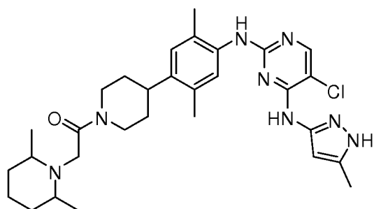
1-(4-(4-(5-chloro-4-(5-methyl-1H-pyrazol-3-ylamino)pyrimidin-2-ylamino)-2,5-dimethylphenyl)piperidin-1-yl)-2-(2,6-dimethylpiperidin-1-yl)ethanone
