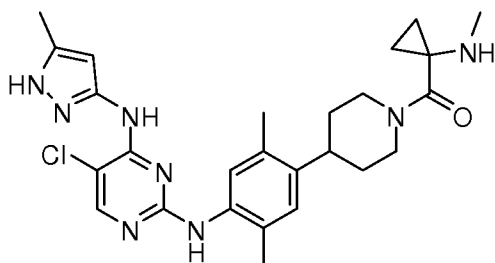
(4-(4-(5-chloro-4-(5-methyl-1H-pyrazol-3-ylamino)pyrimidin-2-ylamino)-2,5-dimethylphenyl)piperidin-1-yl)(1-(methylamino)cyclopropyl)methanone
