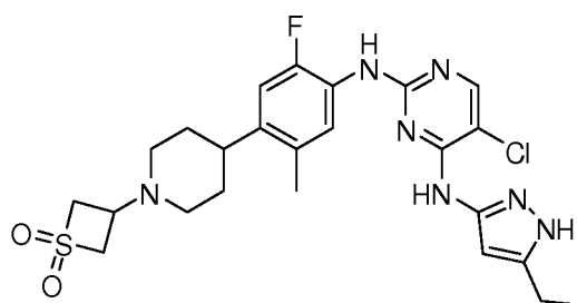
5-Chloro-N2-{4-[1-(1,1-dioxo-1λ6-thietan-3-yl)-piperidin-4-yl]-2-fluoro-5-methylphenyl}-N4-(5-ethyl-1H-pyrazol-3-yl)pyrimidine-2,4-diamine
