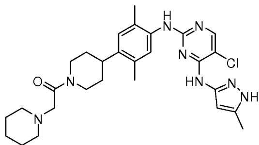
1-(4-(4-(5-chloro-4-(5-methyl-1H-pyrazol-3-ylamino)pyrimidin-2-ylamino)-2,5-dimethylphenyl)piperidin-1-yl)-2-(piperidin-1-yl)ethanone
