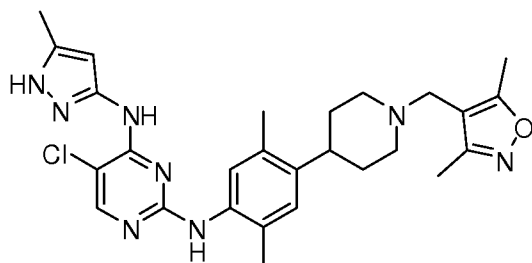
5-chloro-N2-(4-(1-((3,5-dimethylisoxazol-4-yl)methyl)piperidin-4-yl)-2,5-dimethylphenyl)-N4-(5-methyl-1H-pyrazol-3-yl)pyrimidine-2,4-diamine
