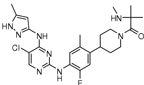
1-(4-(4-(5-chloro-4-(5-methyl-1H-pyrazol-3-ylamino)pyrimidin-2-ylamino)-5-fluoro-2-methylphenyl)piperidin-1-yl)-2-methyl-2-(methylamino)propan-1-one
