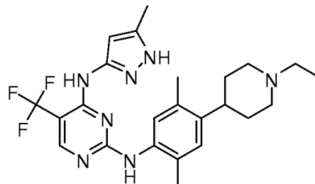
N2-(4-(1-ethylpiperidin-4-yl)-2,5-dimethylphenyl)-N4-(5-methyl-1H-pyrazol-3-yl)-5-(trifluoromethyl)pyrimidine-2,4-diamine
