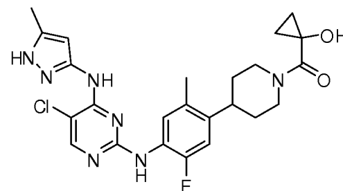
(4-(4-(5-chloro-4-(5-methyl-1H-pyrazol-3-ylamino)pyrimidin-2-ylamino)-5-fluoro-2-methylphenyl)piperidin-1-yl)(1-hydroxycyclopropyl)methanone
