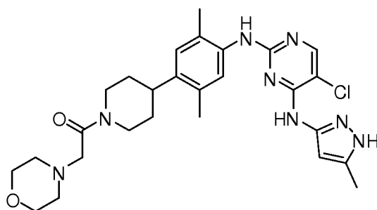
1-(4-(4-(5-chloro-4-(5-methyl-1H-pyrazol-3-ylamino)pyrimidin-2-ylamino)-2,5-dimethylphenyl)piperidin-1-yl)-2-morpholinoethanone
