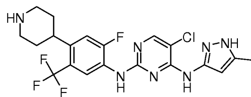
5-chloro-N2-(2-fluoro-4-(piperidin-4-yl)-5-(trifluoromethyl)phenyl)-N4-(5-methyl-1H-pyrazol-3-yl)pyrimidine-2,4-diamine
