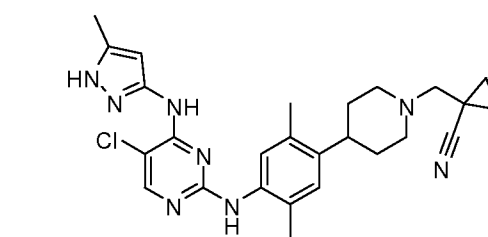
1-((4-(4-(5-chloro-4-(5-methyl-1H-pyrazol-3-ylamino)pyrimidin-2-ylamino)-2,5-dimethylphenyl)piperidin-1-yl)methyl)cyclopropanecarbonitrile
