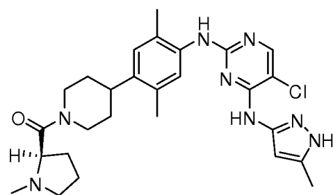
(R)-(4-(4-(5-chloro-4-(5-methyl-1H-pyrazol-3-ylamino)pyrimidin-2-ylamino)-2,5-dimethylphenyl)piperidin-1-yl)(1-methylpyrrolidin-2-yl)methanone
