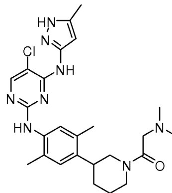
1-(3-(4-(5-chloro-4-(5-methyl-1H-pyrazol-3-ylamino)pyrimidin-2-ylamino)-2,5-dimethylphenyl)piperidin-1-yl)-2-(dimethylamino)ethanone
