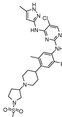
5-chloro-N2-(2-fluoro-5-methyl-4-(1-(1-(methylsulfonyl)pyrrolidin-3-yl)piperidin-4-yl)phenyl)-N4-(5-methyl-1H-pyrazol-3-yl)pyrimidine-2,4-diamine
