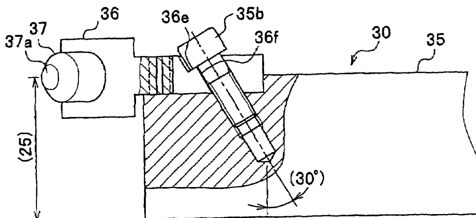
FIG. 4C PRIOR ART
