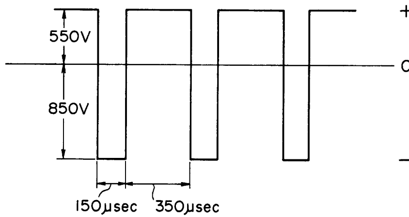
WAVEFORM OF SUPPLY 6
