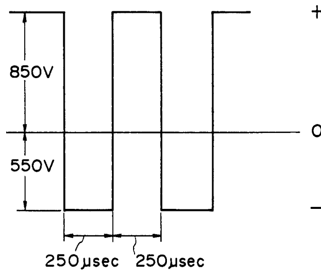
WAVEFORM OF SUPPLY I1
