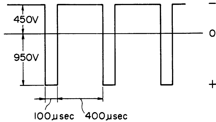
WAVEFORM OF SUPPLY I0
