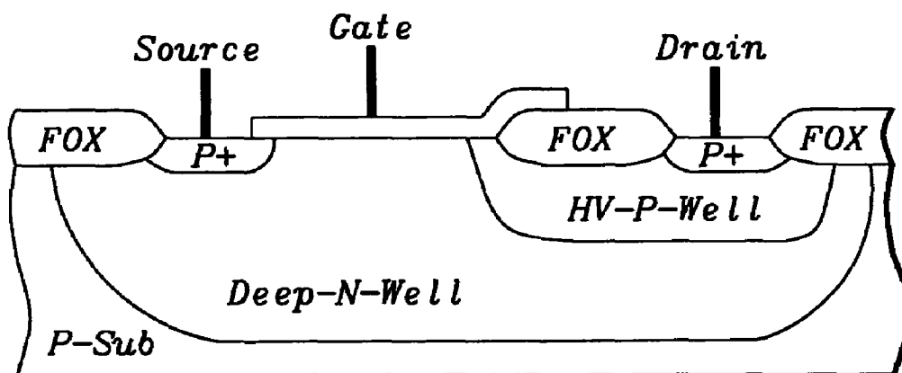
High-Voltage PMOS Cross Section
