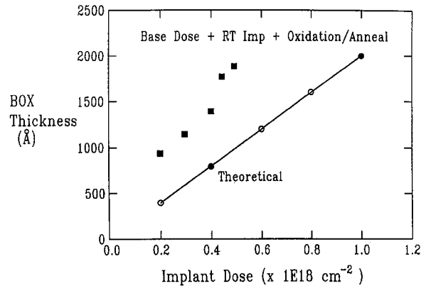
FIG. 2 Thermally Induced BOX via RT Implant
