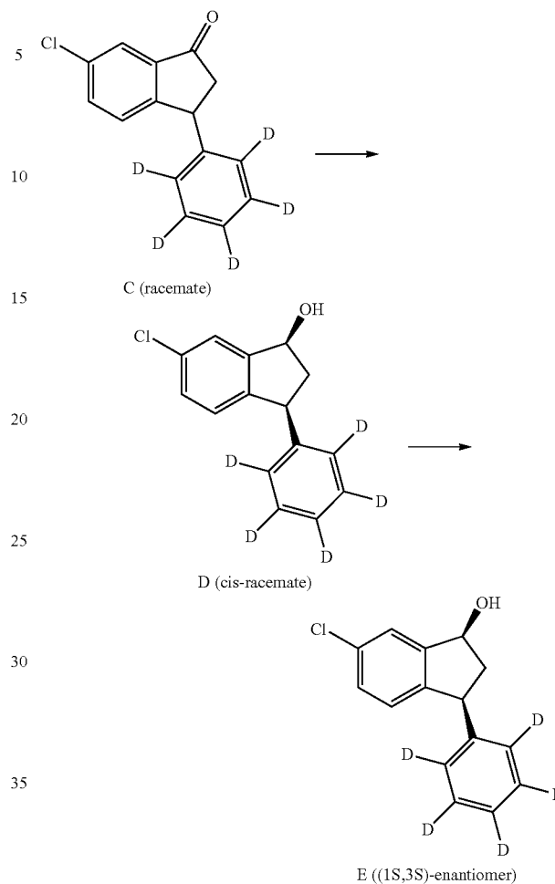
Scheme 2. Exemplary synthesis of intermediate E.
