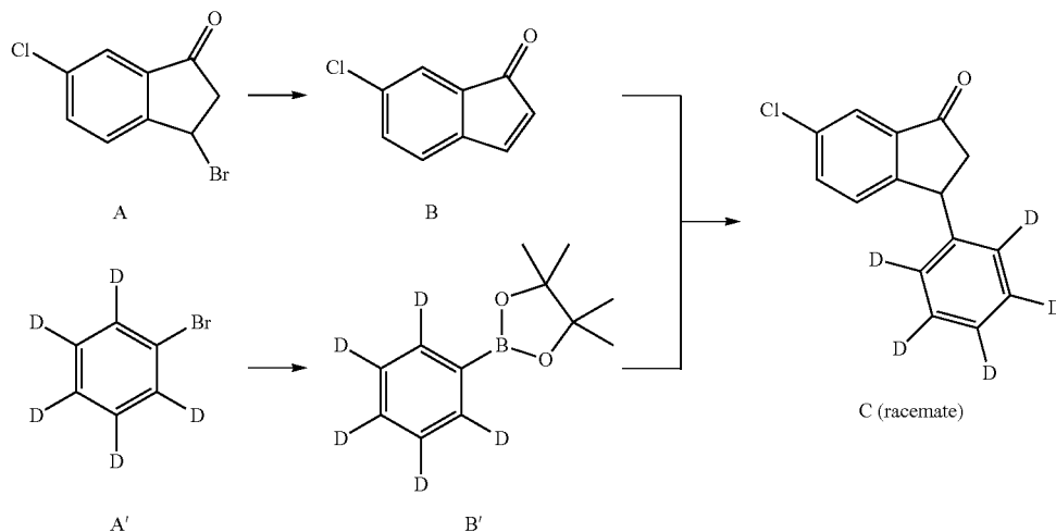
Scheme 9. Synthesis of Compound C.
