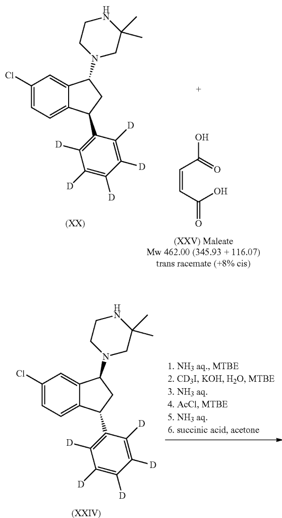
Scheme 17: Synthesis of rac-trans-1-(6-chloro-3-phenyl( d 5 )-indan-1-yl)-1( d 3 ), 2,2-trimethyl-piperazine succinate
