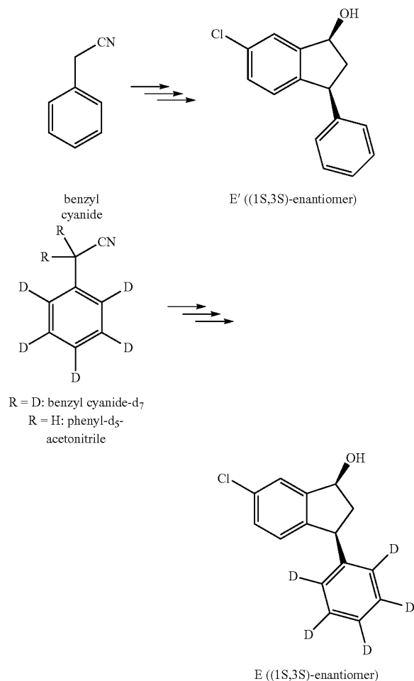
Scheme 4. Exemplary synthesis of intermediate E and E'.
