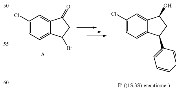
Scheme 3. Exemplary synthesis of intermediate E'.
