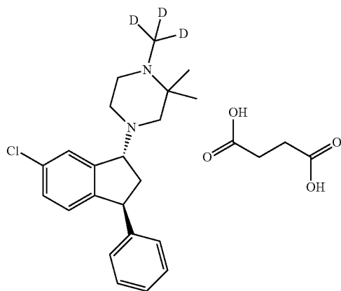
Compound (I) butanedioic acid salt
