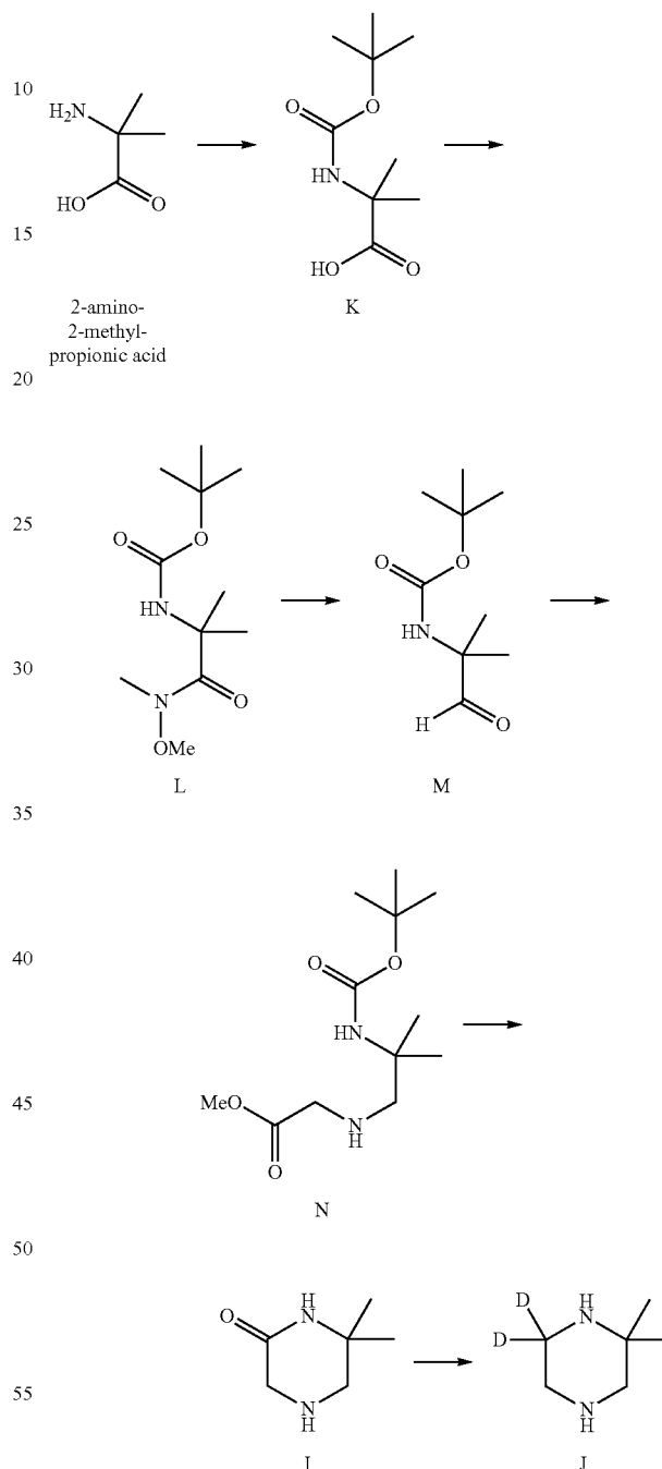
Scheme 7. Alternative exemplary synthesis of intermediate J.
