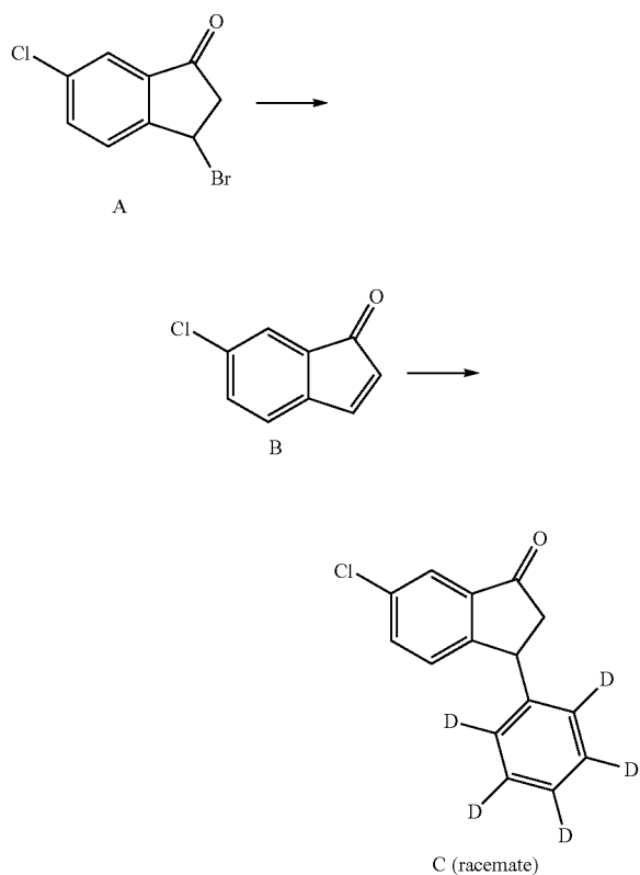
Scheme 1. Exemplary synthesis of intermediate C.
