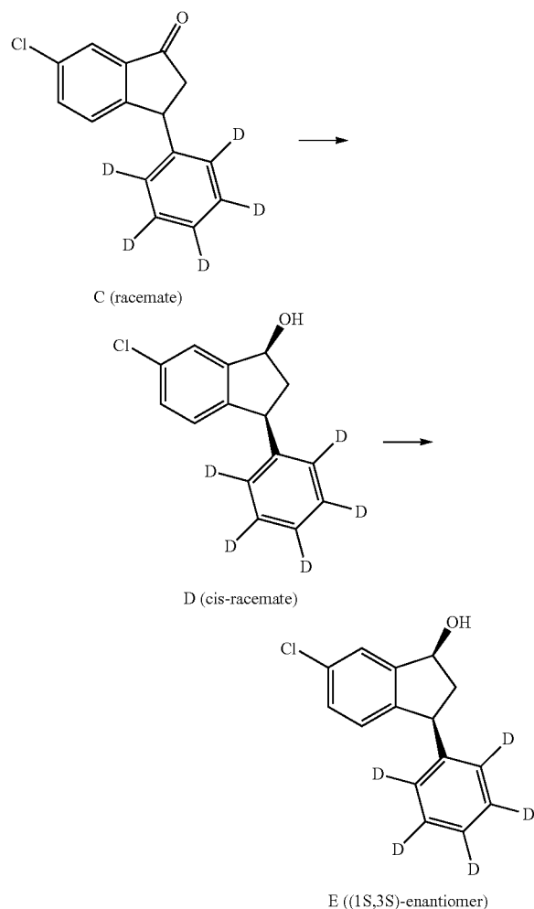
Scheme 10. Synthesis and resolution of Compound E.
