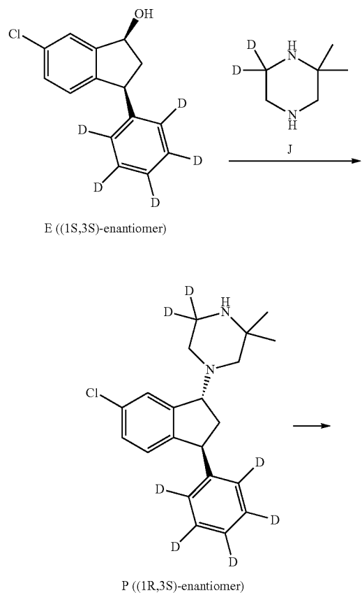
Scheme 13. Synthesis of Compound (VI) and Compound (VII).
