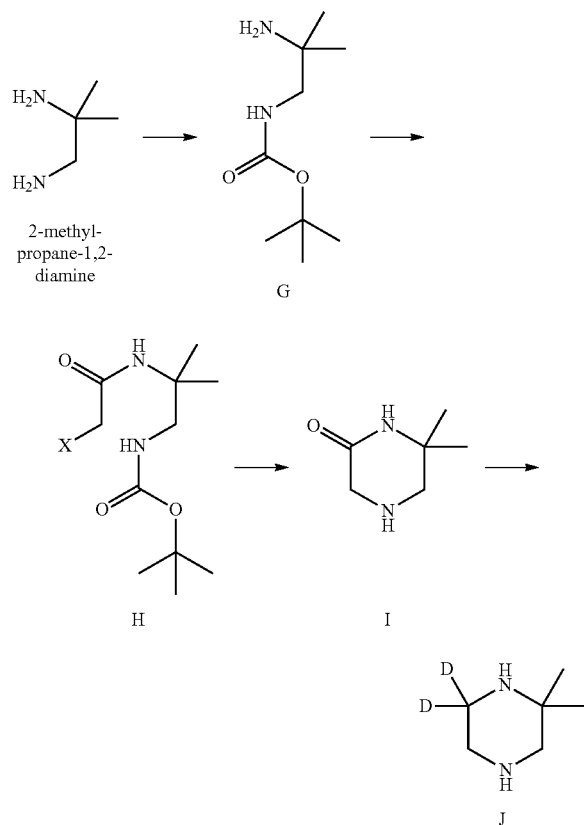
Scheme 6. Exemplary synthesis of intermediate J.
