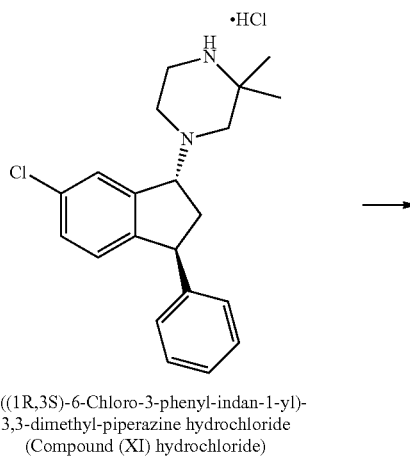
Scheme 8. Synthesis of Compound (I).
