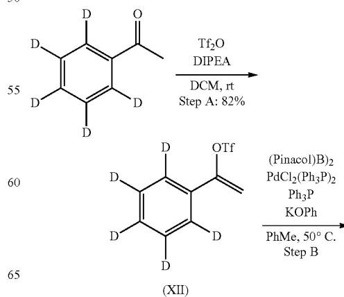
Scheme 14. Synthesis of Compound (XV)
