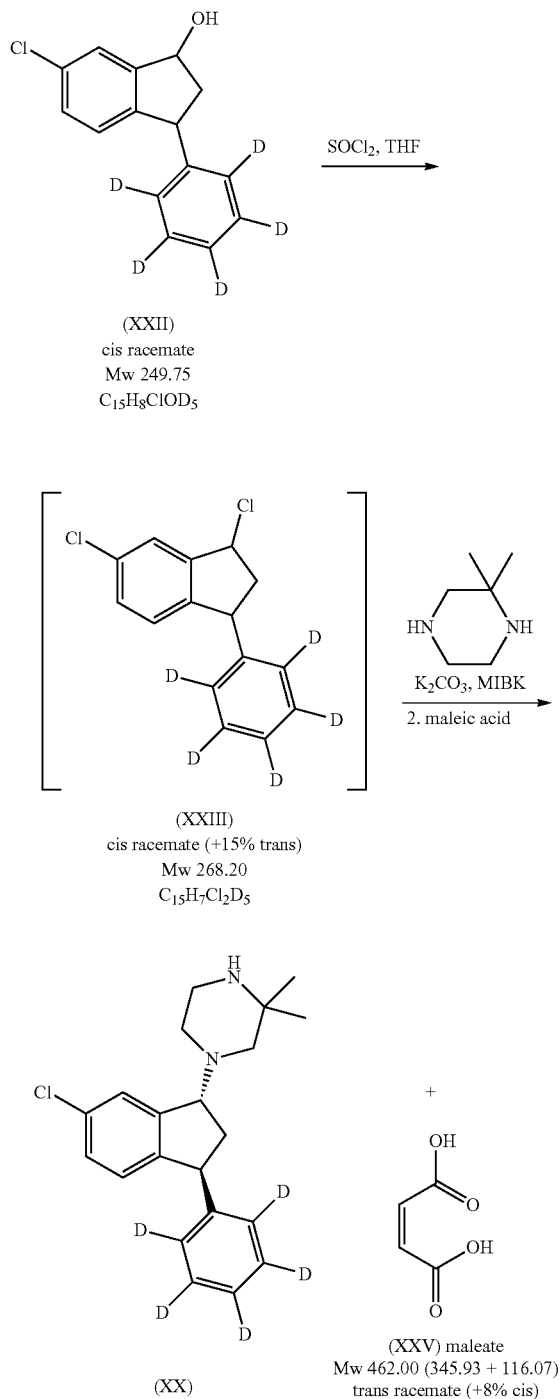
Scheme 16: Synthesis of rac-trans-1-(6-Chloro-3-phenyl( d_5 )-indan-1-yl)-3,3-dimethyl-piperazine maleate
