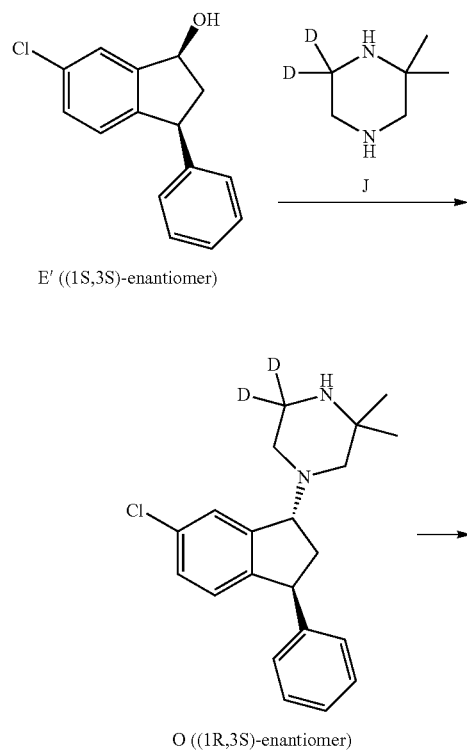
Scheme 12. Synthesis of Compound (III) and Compound (V).
