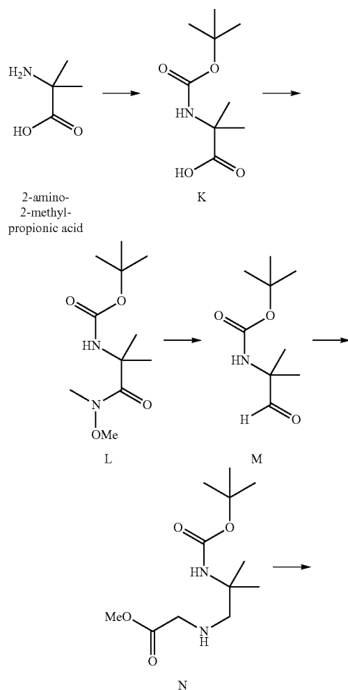
Scheme 11. Synthesis of intermediate J.
