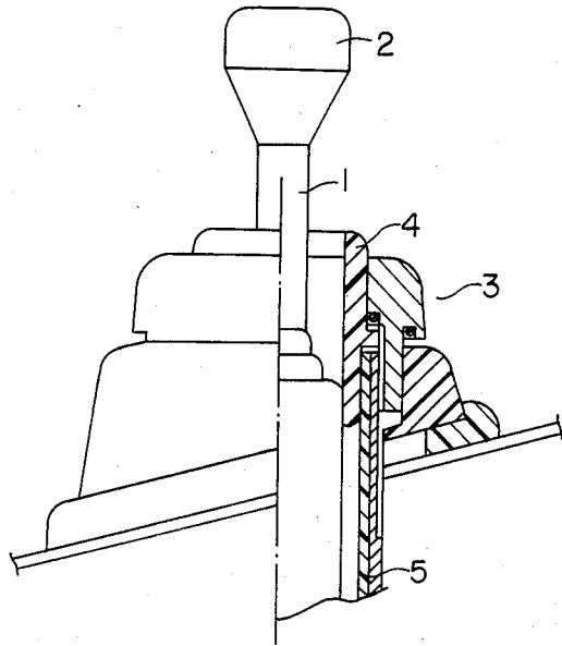
FIG. 2 PRIOR ART
