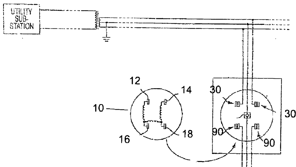
Figure 2 (Prior Art)
