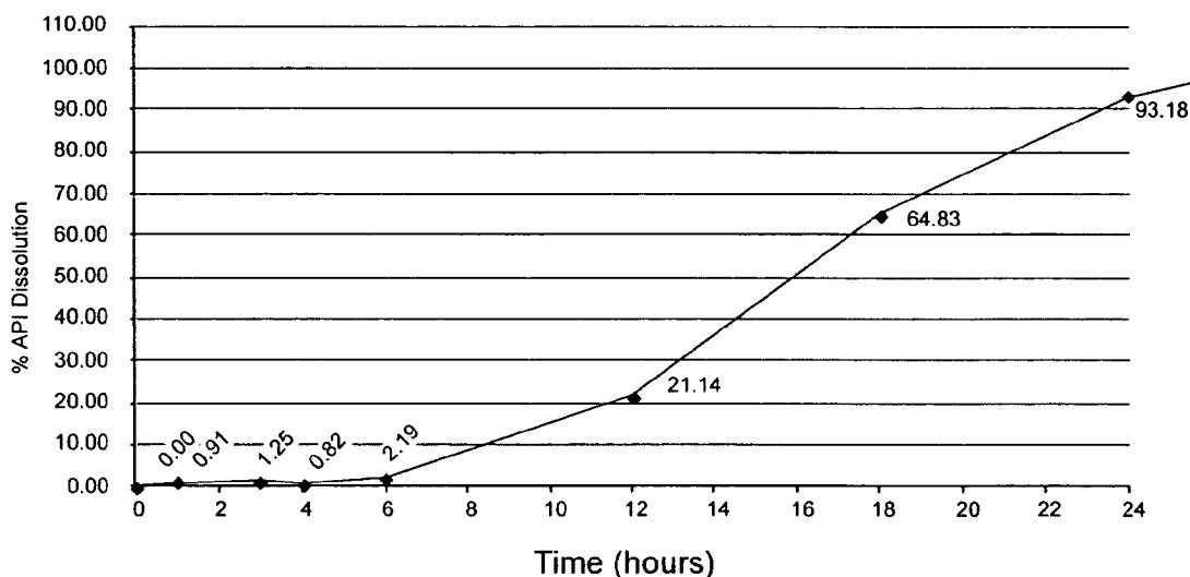
Cyclosporin A dissolution from minicapsules coated with 22% Eudrgit RS30D
