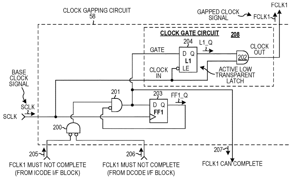
A CLOCK GAPPING CIRCUIT (FOR CPU#1)
