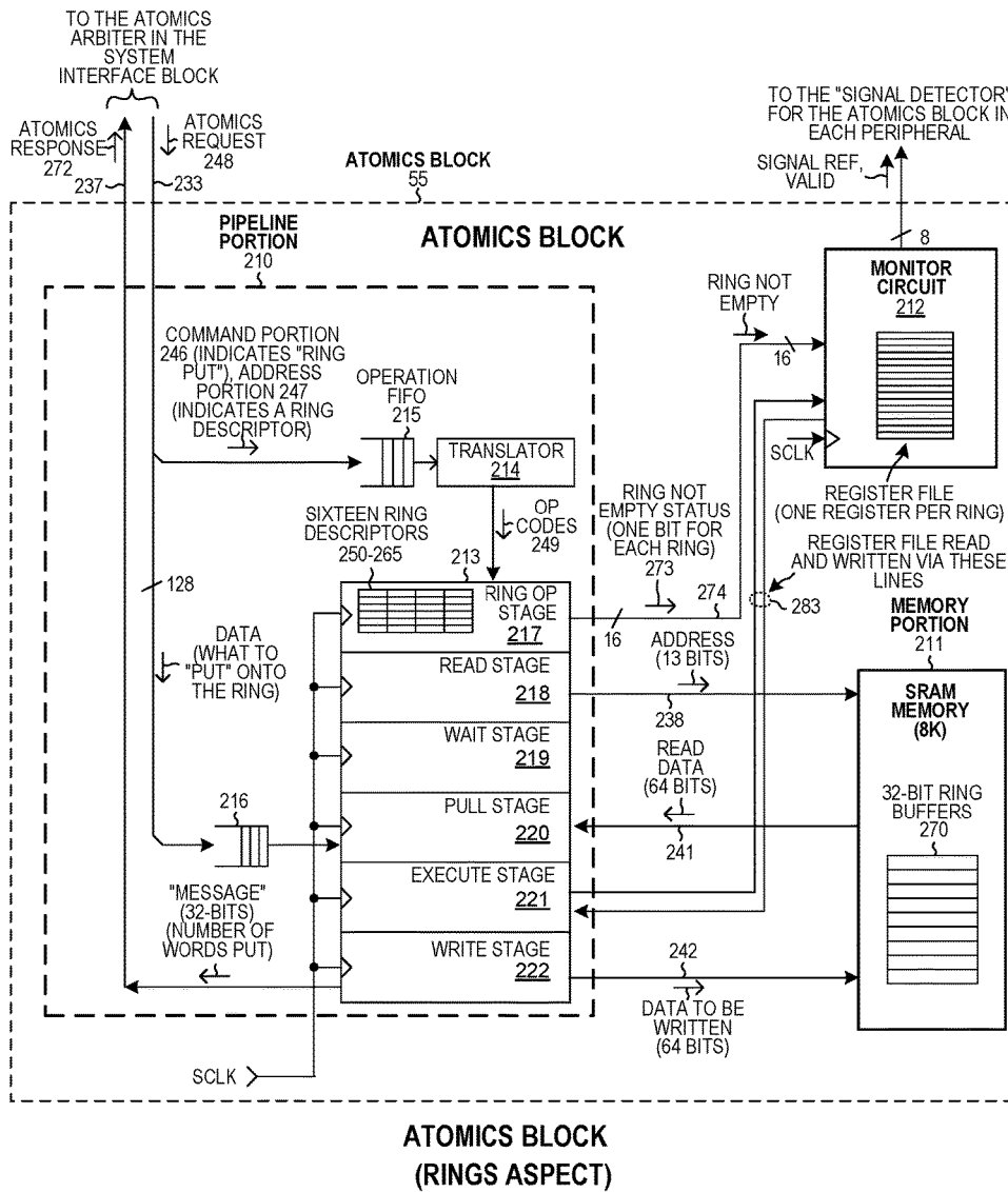
ATOMICS BLOCK (RINGS ASPECT)
