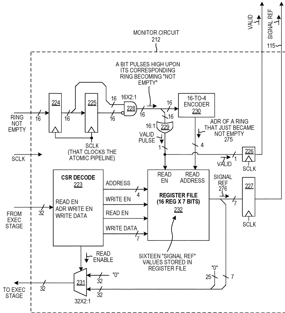
MONITOR CIRCUIT FIG. 23
