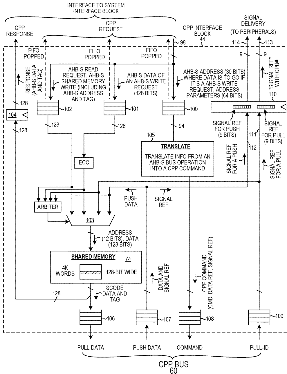
CPP INTERFACE BLOCK
