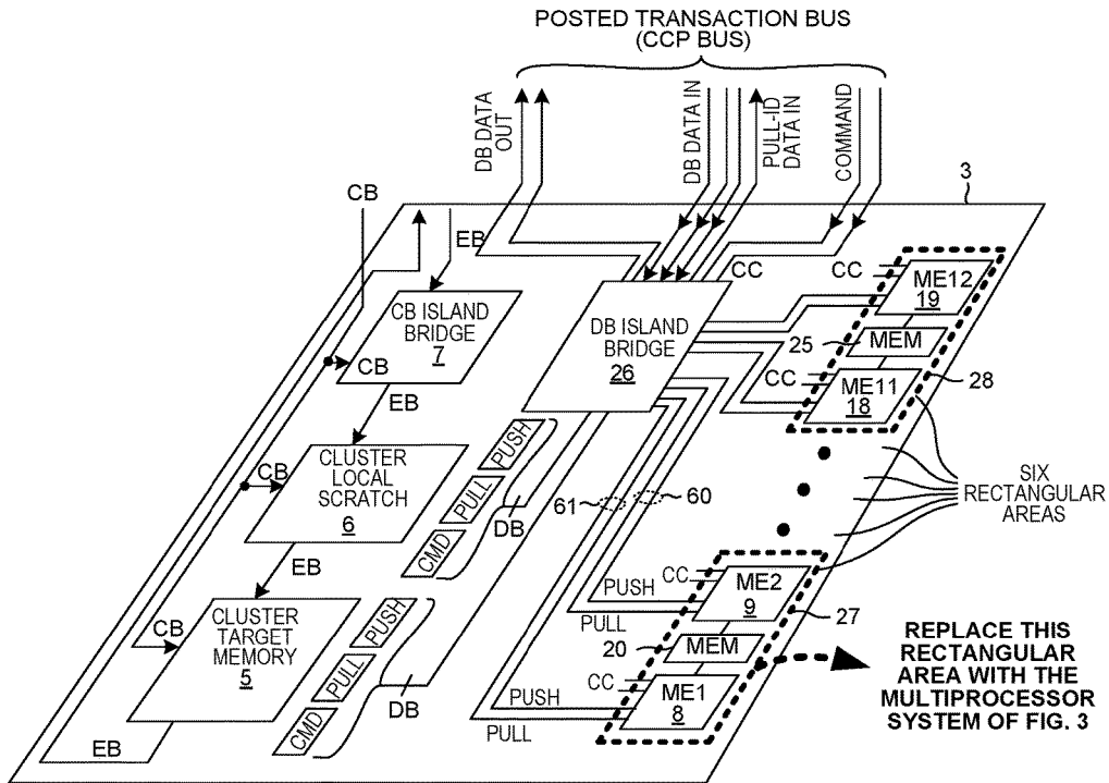
MICROENGINE (ME) ISLAND FIG. 2
