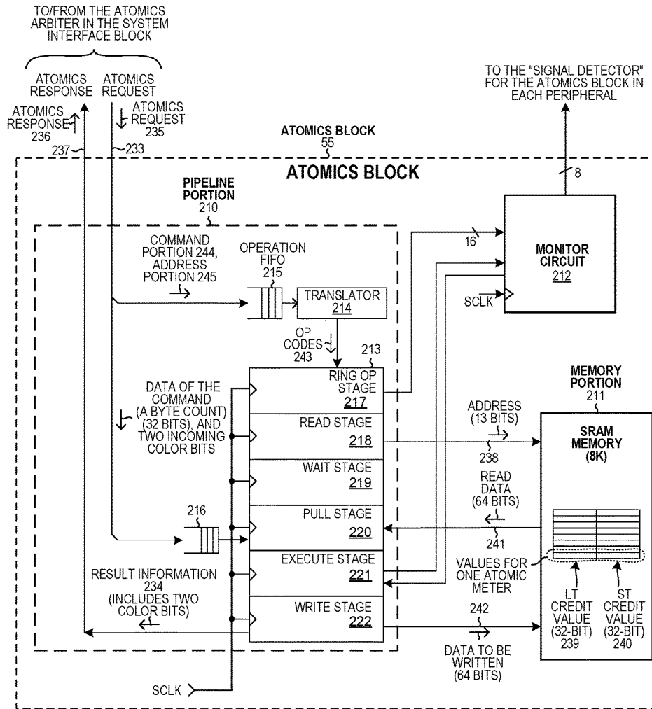
ATOMICS BLOCK (ATOMIC METERING ASPECT)
