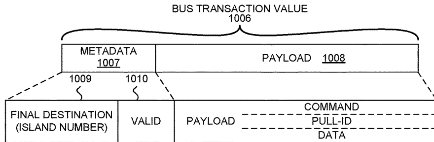
META DATA AND PAYLOAD FIG. 30
