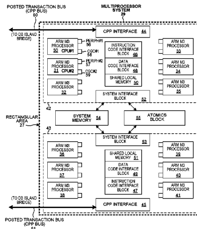
MULTIPROCESSOR SYSTEM
