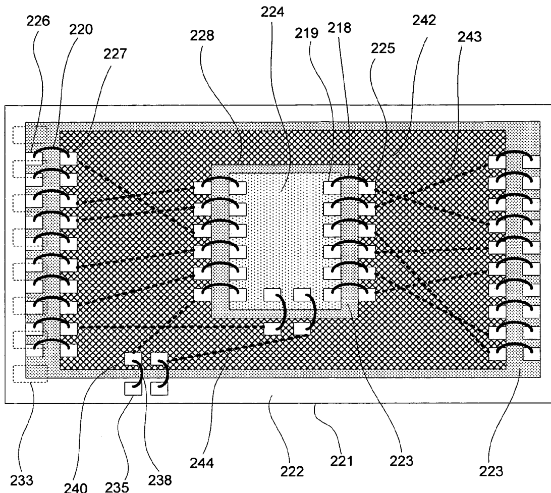
Invention (Top View)
