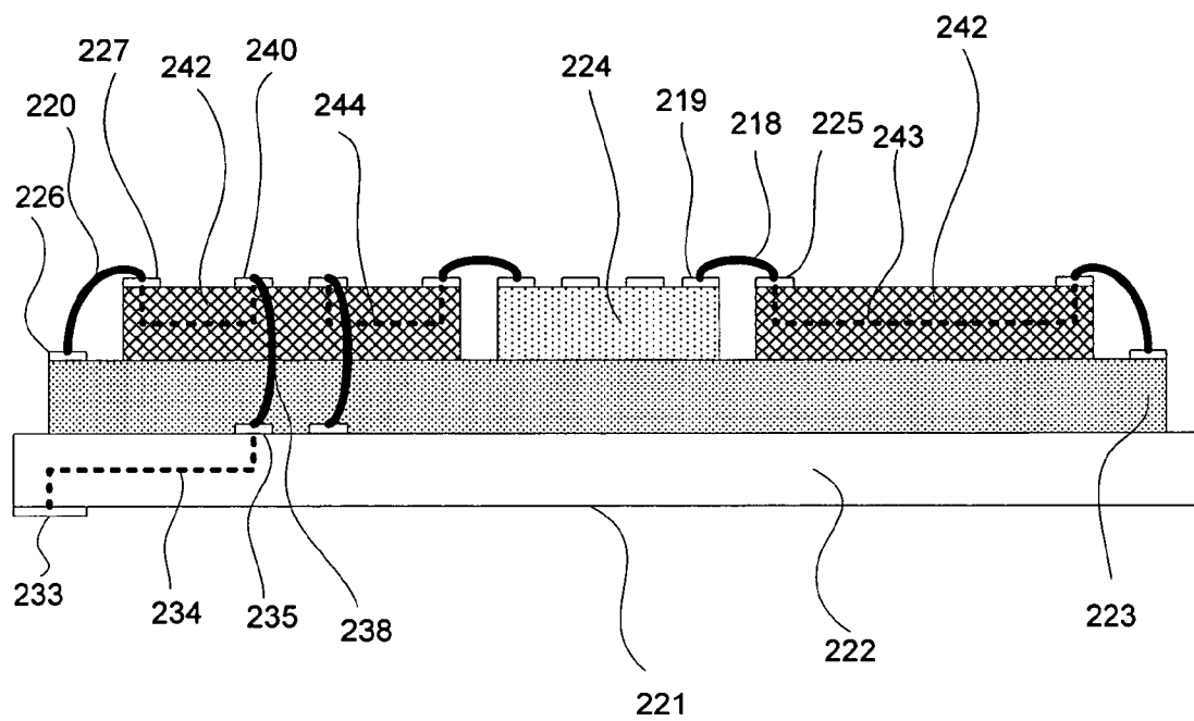
FIG-7 Invention (Cross Section View)
