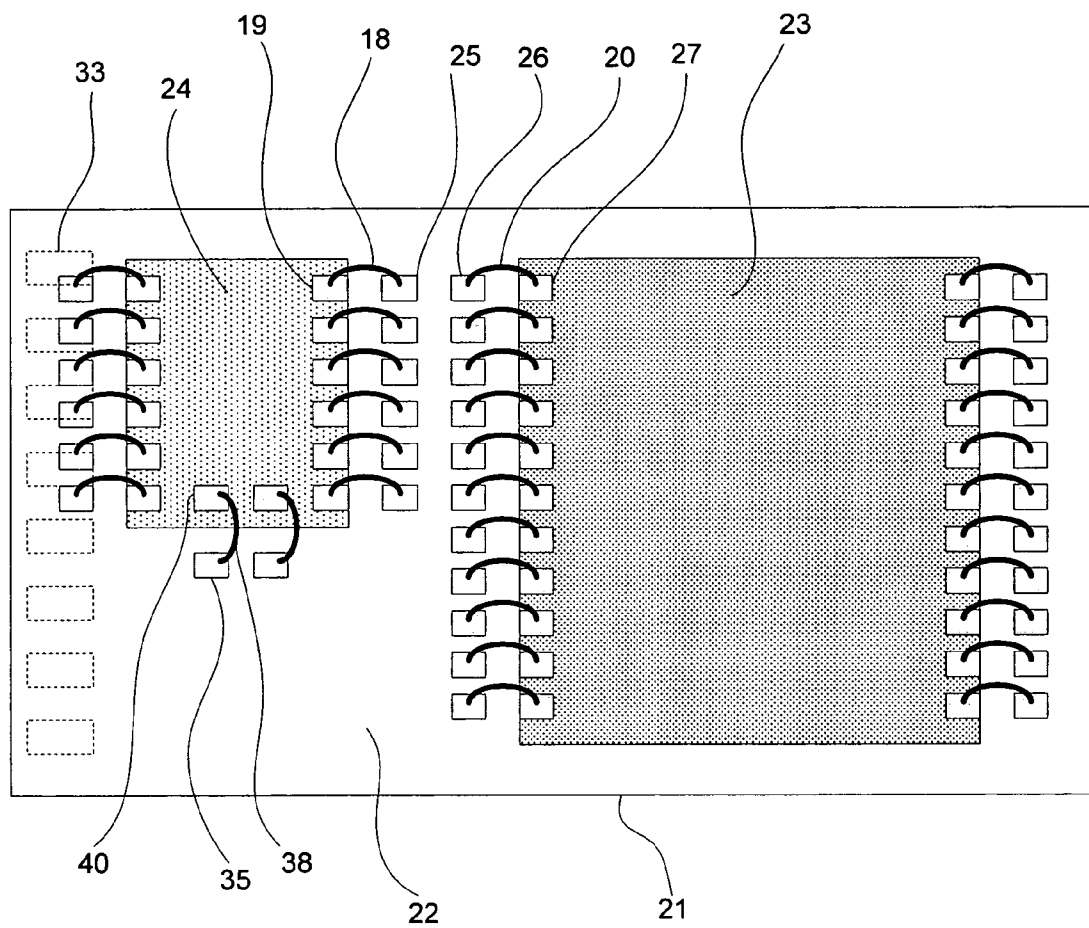
FIG-2 Prior Art (Top View)
