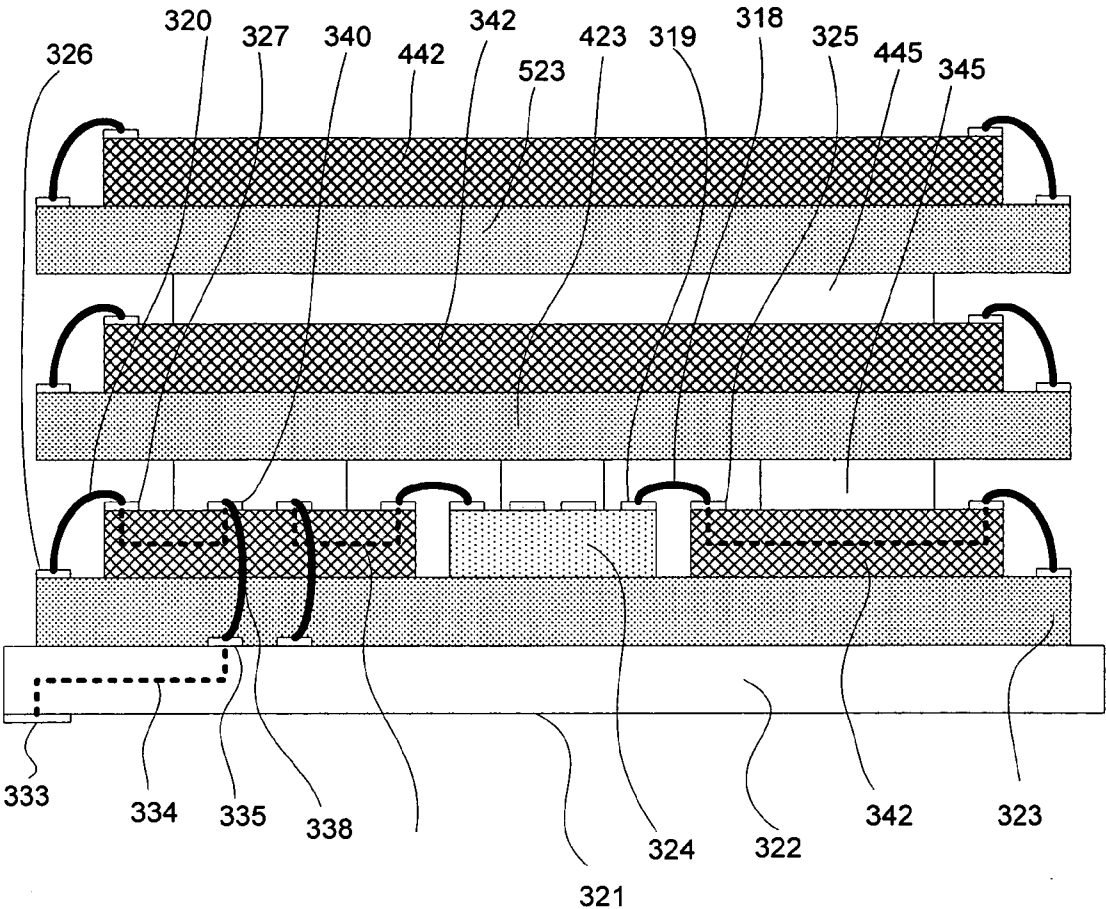
FIG-10 (Cross Section View)
