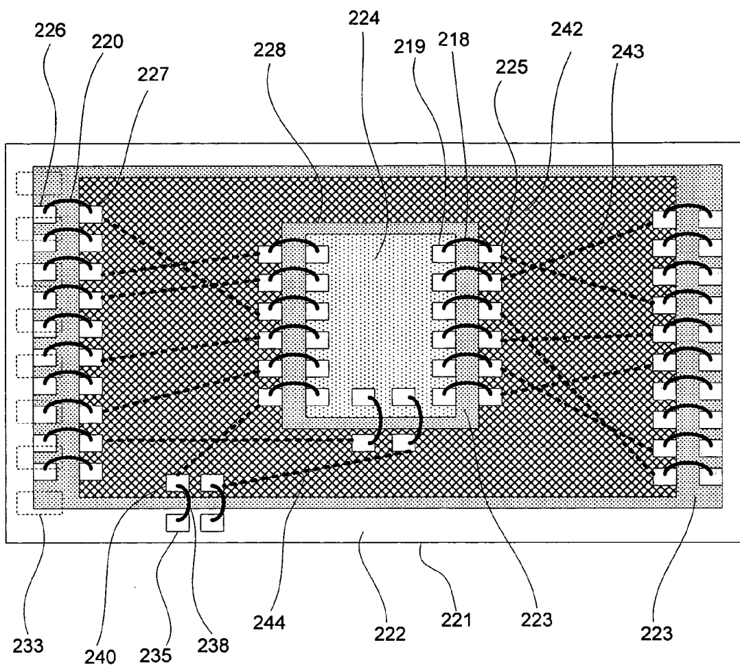
FIG-6 Invention (Top View)
