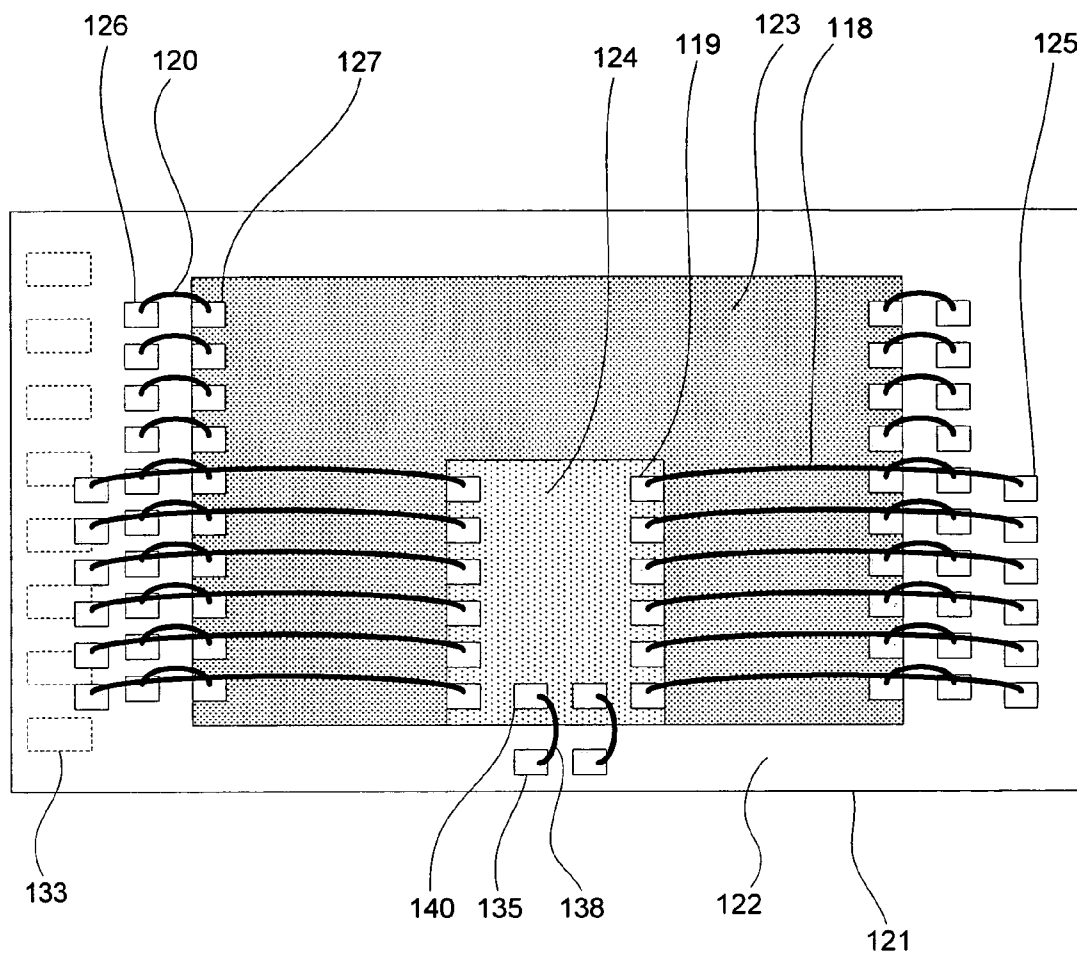
FIG-4 Prior Art – STACKING (Top View)
