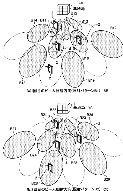
AA Base station BB (a) Direction of first beam irradiation (irradiation pattern B1) CC (b) Direction of second beam irradiation (irradiation pattern B2)
