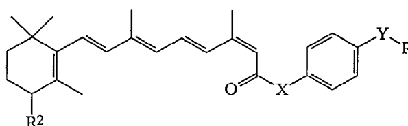
Formula 1, 13- cis
