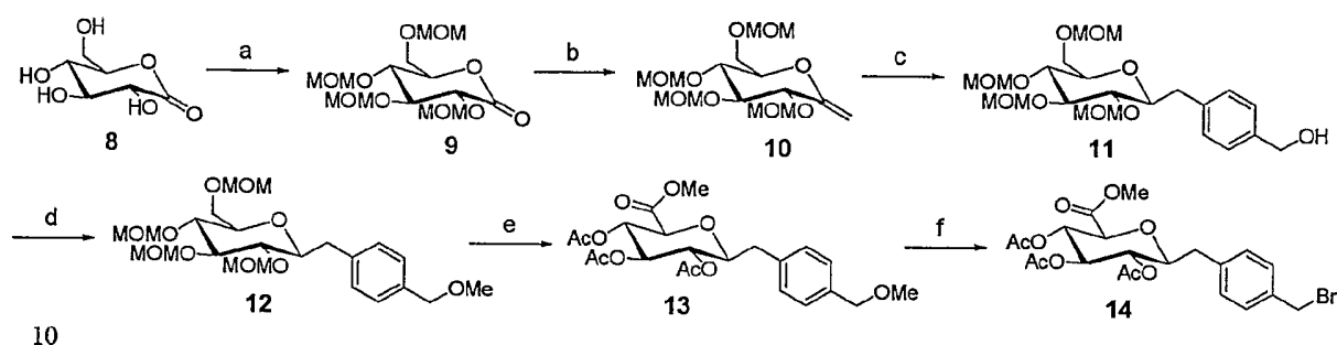
REACTION SCHEME 1
