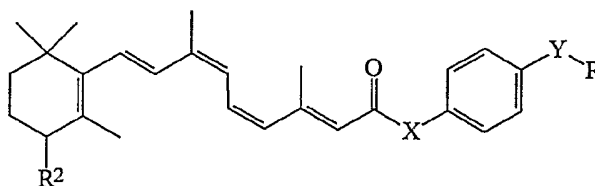
Formula 1, 9- cis
