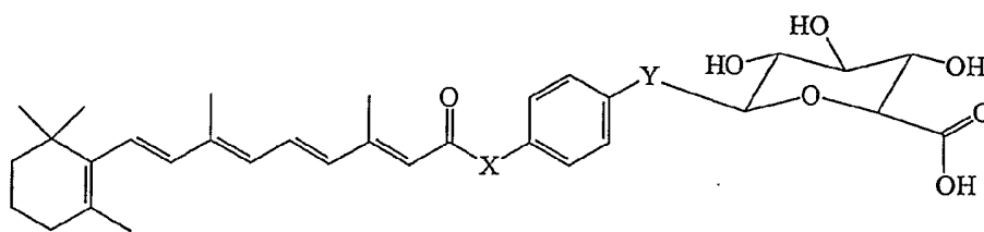
4-HBRCG
