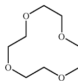
18-crown-6-ether
