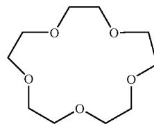
15-crown-5-ether
