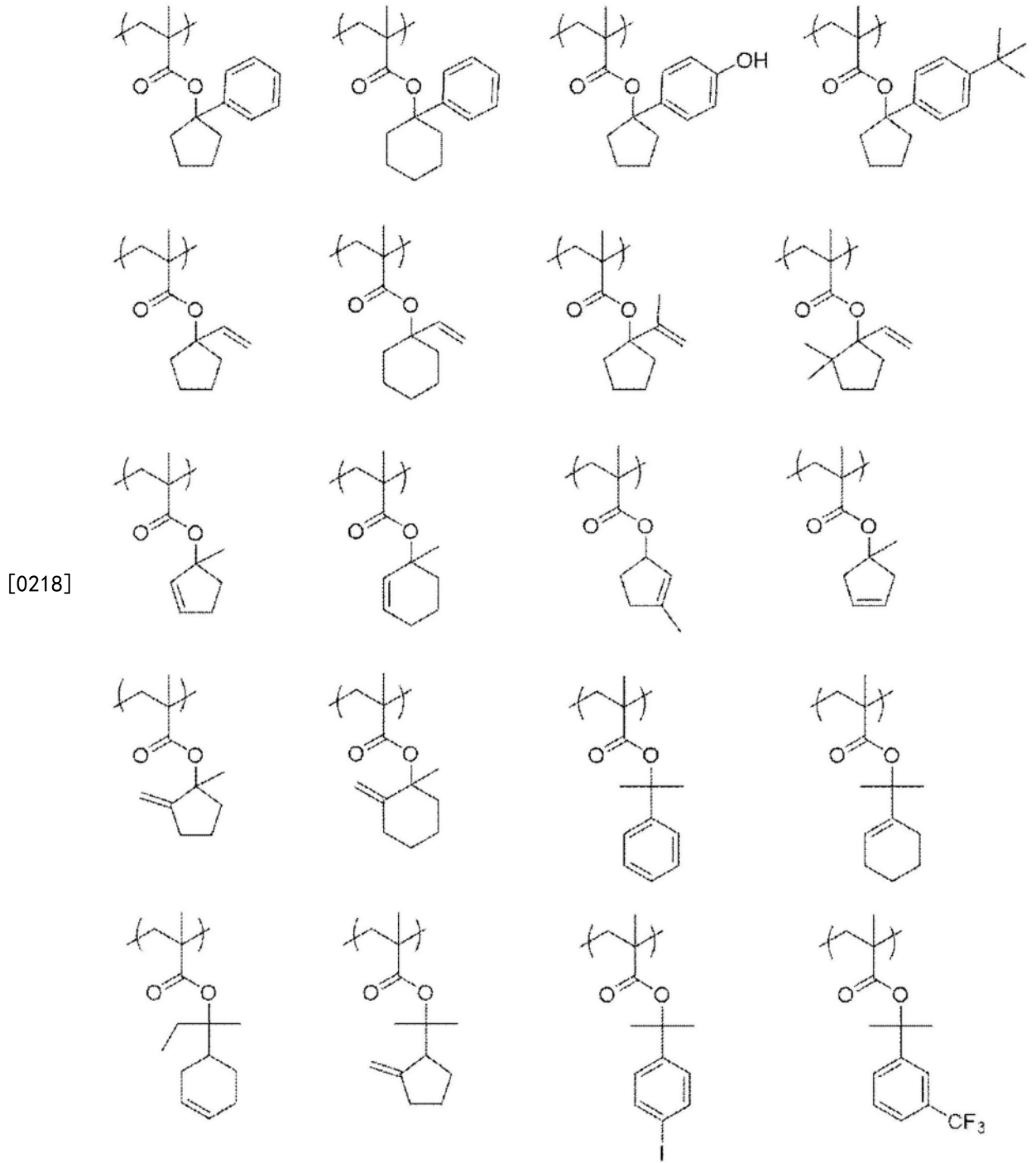
[0219] [化学式13]
